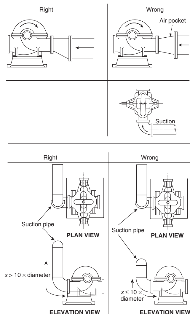
FIGURE A.5.14.6 Right and Wrong Pump Suctions.
