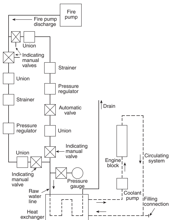
FIGURE A.11.2.6.3 Cooling Water Line with Bypass.
