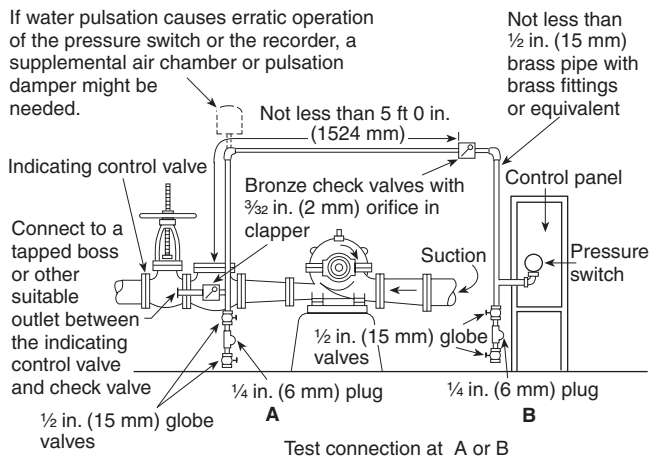
FIGURE A.10.5.2.1(b) Piping Connection for Pressure-Sensing Line (Electric Fire Pump).
