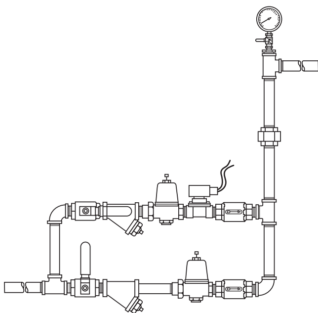
FIGURE A.11.2.6.3.1.4(A) Spring-Loaded Check Valve Arrangement.
