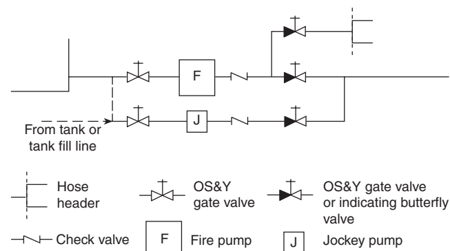
FIGURE A.5.24.4 Jockey Pump Installation with Fire Pump.
