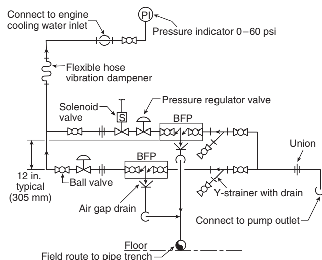
FIGURE A.11.2.6.3.1.4(B) Backflow Preventer Arrangement.
