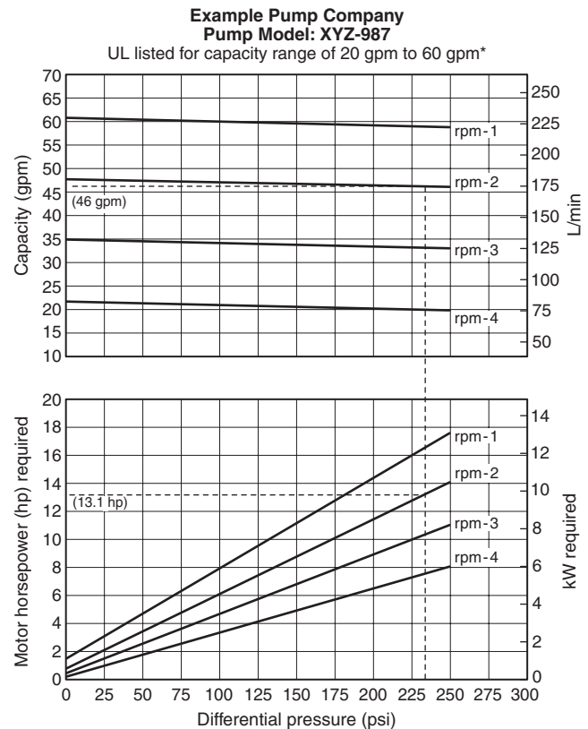
FIGURE A.8.1.2.2 Example of Positive Displacement Pump Selection.
