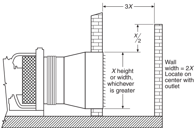
FIGURE A.11.3.2.4 Typical Wind Wall.
