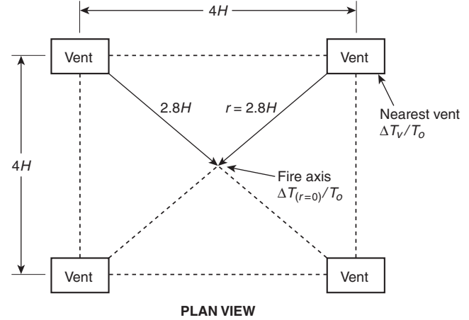
Figure A.5.4.2 Vent Spacing in Rectangular Matrix, When r = 2.8H , (\Delta T_v/T_o) = 0.5 (\Delta T(r=0)/T_o) (plan view).
