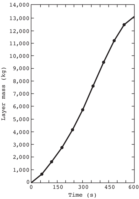
Figure D.10(e) Layer Mass.
