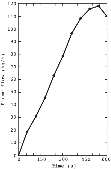
Figure D.10(f) Plume Flow.
