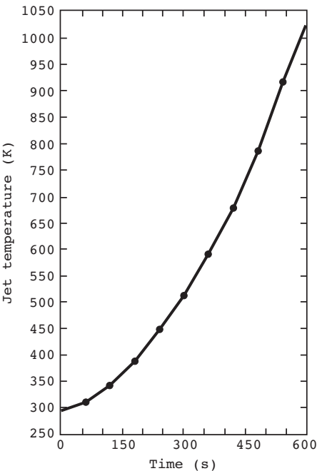
Figure D.10(h) Jet Temperature.
