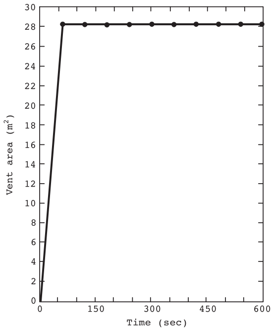
Δ FIGURE D.10(d) Vent Area.
