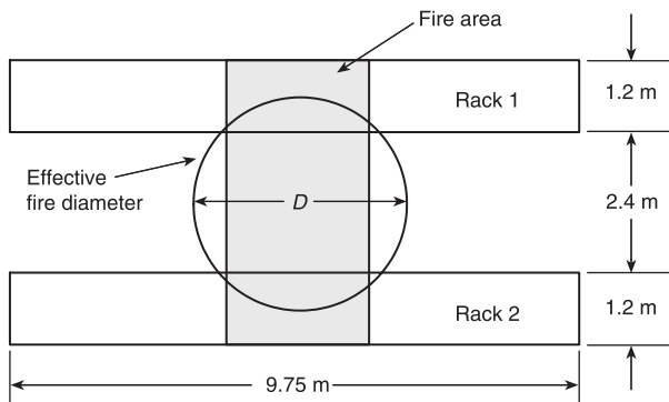
FIGURE D.6 Effective Fire Diameter.
