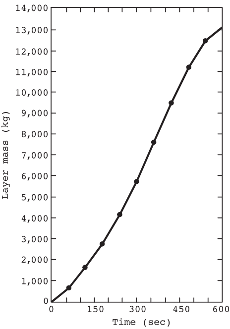
Δ FIGURE D.10(e) Layer Mass.
