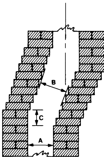
Figure 3-1.2(a) Corbels for Supporting Chimneys.
