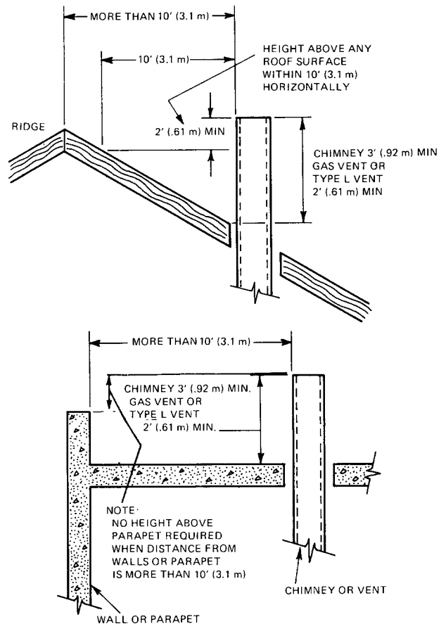
Termination more than 10 feet (3.1 m) from ridge, wall or parapet.
