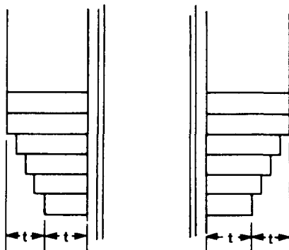
Figure 3-1.2(c) Corbels to Increase Chimney Wall Thickness.
