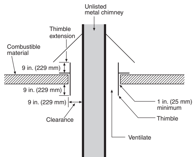
FIGURE 8.2.2.2.7 Ventilating Thimble.
