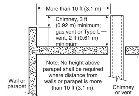
FIGURE 4.2(b) Chimney or Vent Termination More Than 10 ft (3.1 m) from Ridge, Wall, or Parapet.
