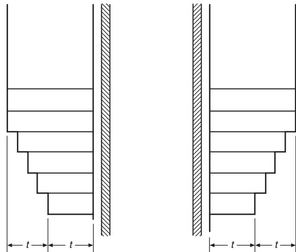
FIGURE 7.1.2(b) Corbels to Change Chimney Direction.
