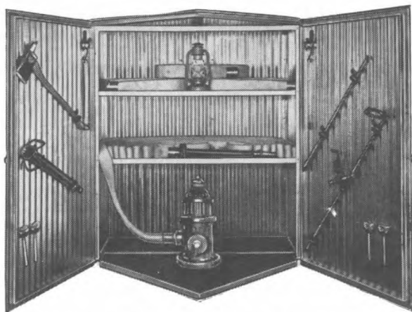
FIG. 53-3. TYPICAL METAL HOSE HOUSE FOR EQUIPMENT DETAILS SEE SECTIONS 55-58
