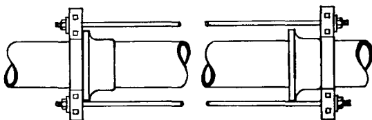
FIG. 96-2. PIPE ANCHOR
