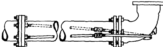
FIG. 96-34. BEND ANCHOR TO FLANGE SPIGOT
