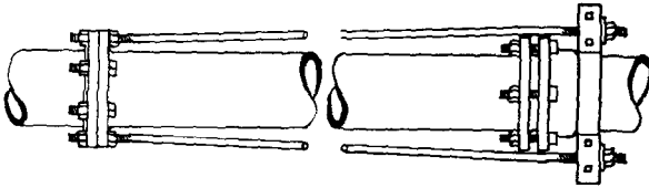
FIG. 96-32. PIPE ANCHOR TO FLANGE SPIGOT
