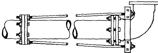
FIG. 96-33. BEND ANCHOR TO FLANGE SPIGOT
