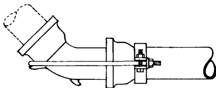
FIG. 96-5. ANCHOR FOR \frac{1}{8} BEND SPIGOT END
