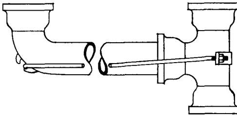
FIG. 96-17. ANCHOR FOR BELL END TEE AND \frac{1}{4} BEND SPIGOT END
