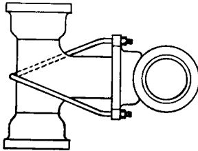
FIG. 96-30. HYDRANT ANCHOR TO SPIGOT TEE
