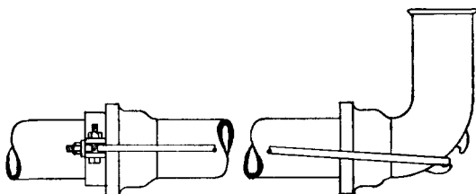
FIG. 96-6. ANCHOR FOR \frac{1}{4} BEND BELL END If distance between joints shown is less than 12 feet, see Note 1.
