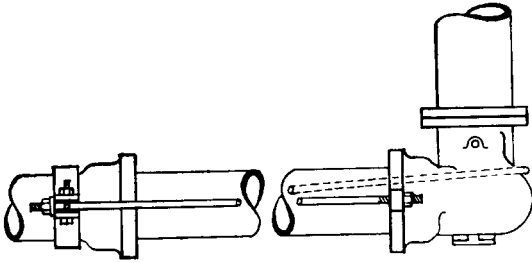
FIG. 96-29. HYDRANT ANCHOR TO PIPE
