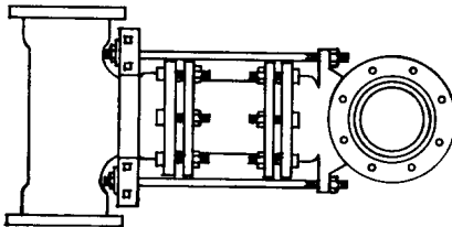
FIG. 96-31. HYDRANT ANCHOR TO TEE BELL WITH SPIGOT PIECE
