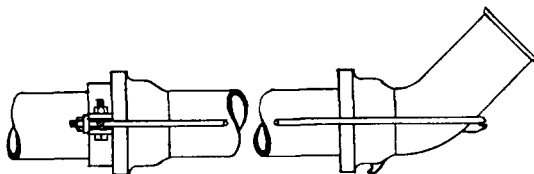
FIG. 96-7. ANCHOR FOR \frac{1}{8} BEND BELL END If distance between joints shown is less than 12 feet, see Note 1.
