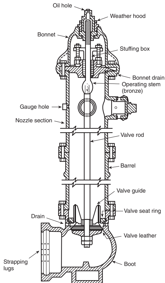
Figure 1-5(b) Dry barrel hydrant.
