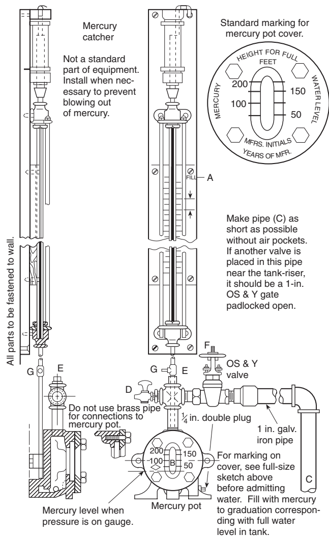
Figure A-6-3.1 Mercury gauge.
