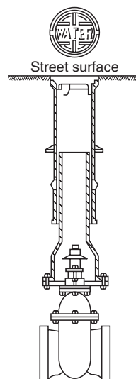
Figure A-9-1(m)(2) Nonindicating-type gate valve.
