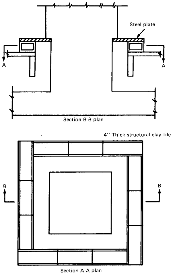
Figure 4-2 Installation of Downflow Furnace on Combustible Floor.
