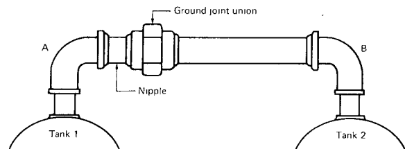
Figure 2-2 This shows the detail of the cross connection which can be used in Figure 2-2.
