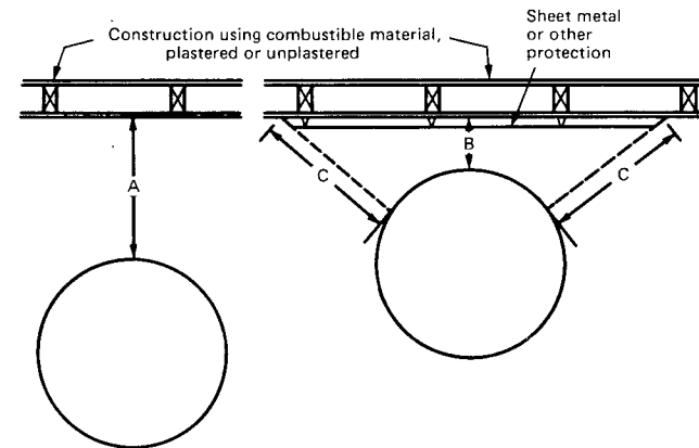
Figure B-1 Clearances with Specified Forms of Protection.
