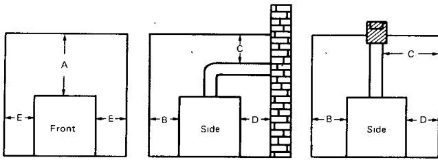
Figure 4-1 Clearances to Combustible Materials.
