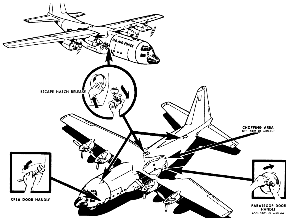
Figure B-15. Emergency entrance into the USAF C-130A troop transport.
