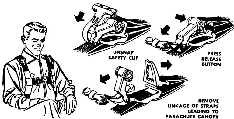
Figure B-4. Release mechanism on one type canopy release type harness.
