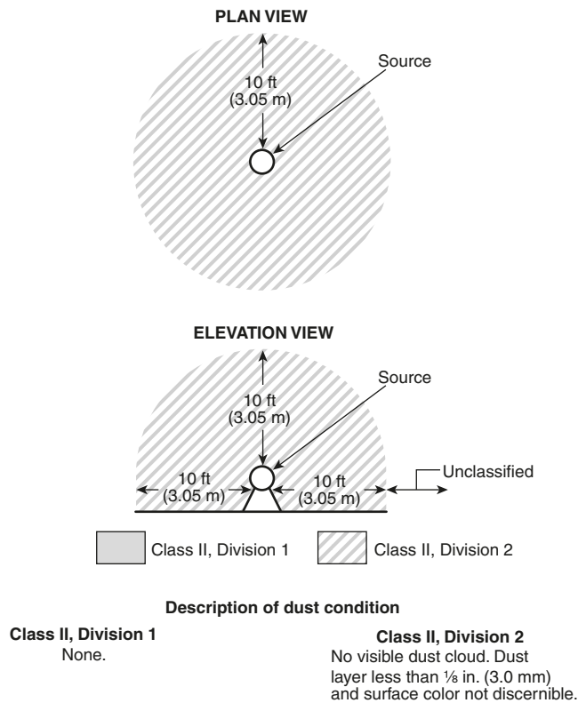
Δ FIGURE 6.10(c) Group F or Group G Dust — Indoor, Unrestricted Area; Operating Equipment Enclosed; Area Classified as a Class II, Division 2 Location.
