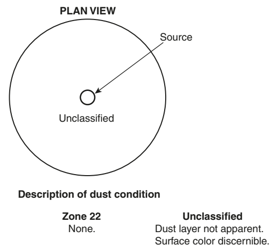
FIGURE 6.10(n) Zone Group IIIB or IIIC Dust — Storage Area; Bags, Drums, or Closed Hoppers.
