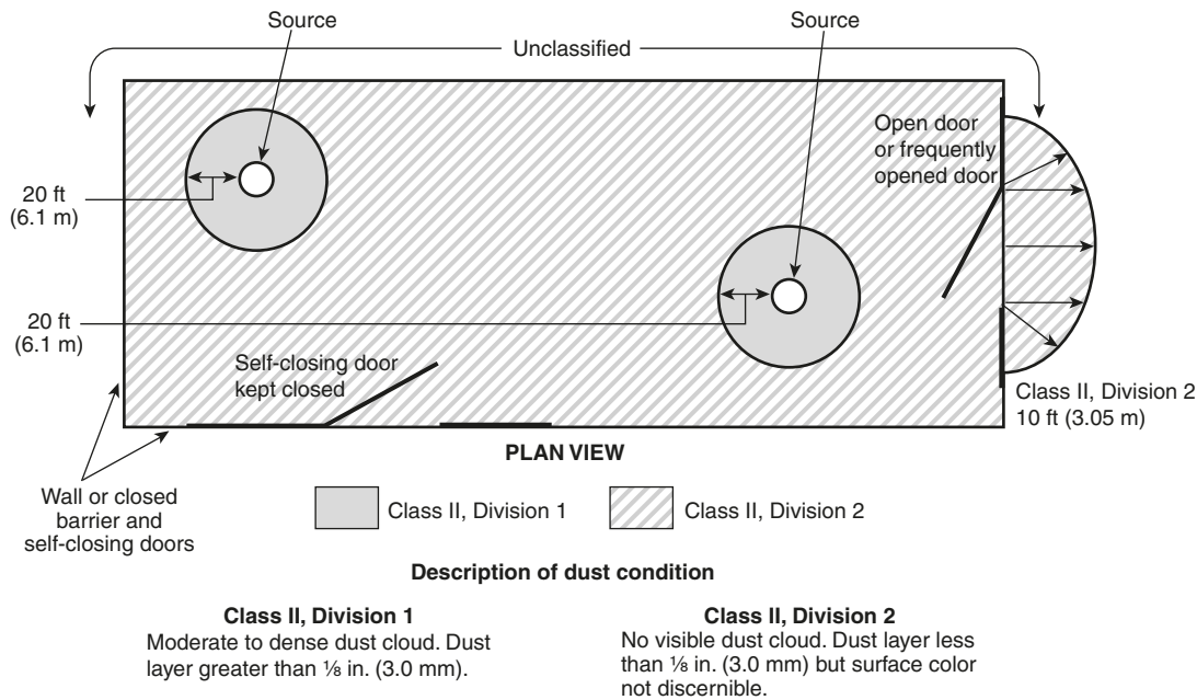
▲ FIGURE 6.10(h) Group F or Group G Dust — Indoor, Walled-Off Area; Multiple Pieces of Operating Equipment.
