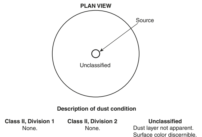
Δ FIGURE 6.10(e) Groups E, F, or G Dusts — Storage Area Bags, Drums, or Closed Hoppers.
