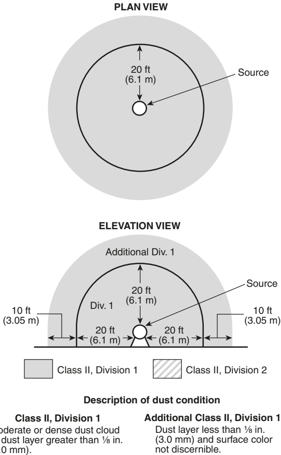
Δ FIGURE 6.10(b) Group E Dust — Indoor, Unrestricted Area; Open or Semi-Enclosed Operating Equipment.
