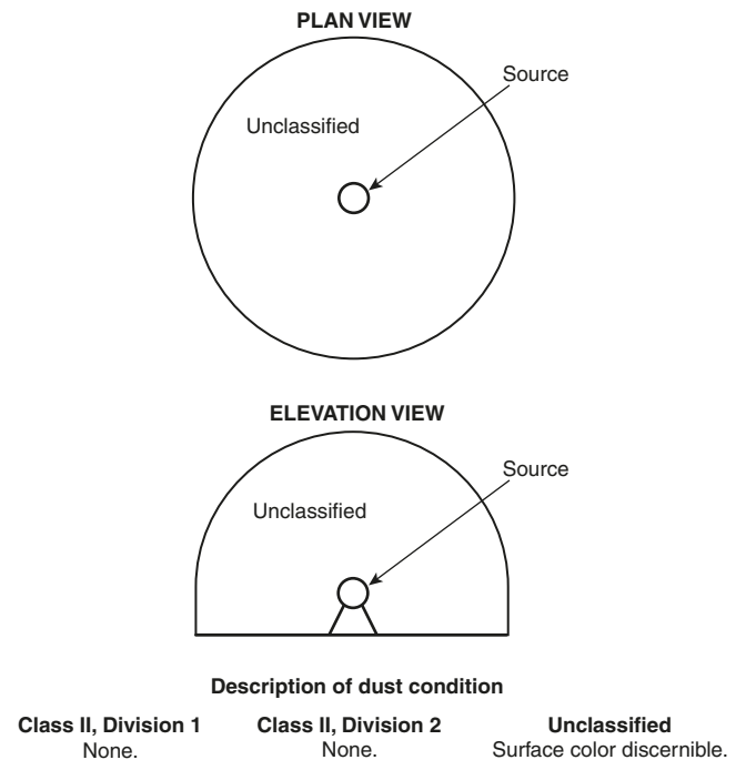
Δ FIGURE 6.10(d) Group F or Group G Dust — Indoor, Unrestricted Area; Operating Equipment Enclosed; Area is an Unclassified Location.
