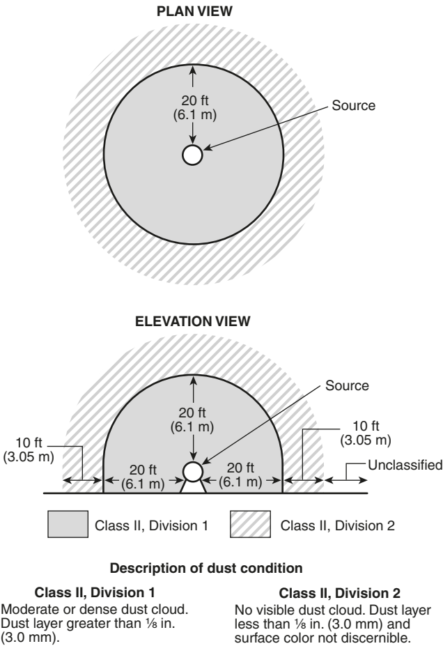
Δ FIGURE 6.10(a) Group F or Group G Dust — Indoor, Unrestricted Area; Open or Semi-Enclosed Operating Equipment.
