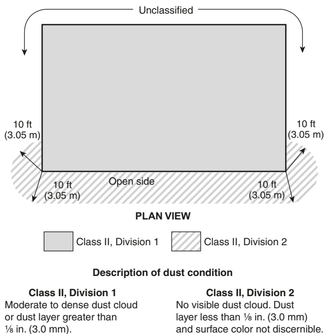
▲ FIGURE 6.10(i) Group F or Group G Dust — Indoor, Unrestricted Area; Ventilating Bagging Head.
