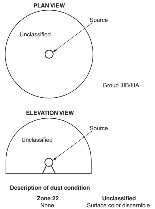
FIGURE 6.10(m) Zone Group IIIB Dust — Indoor, Unrestricted Area; Operating Equipment Enclosed; Area Is an Unclassified Location.
