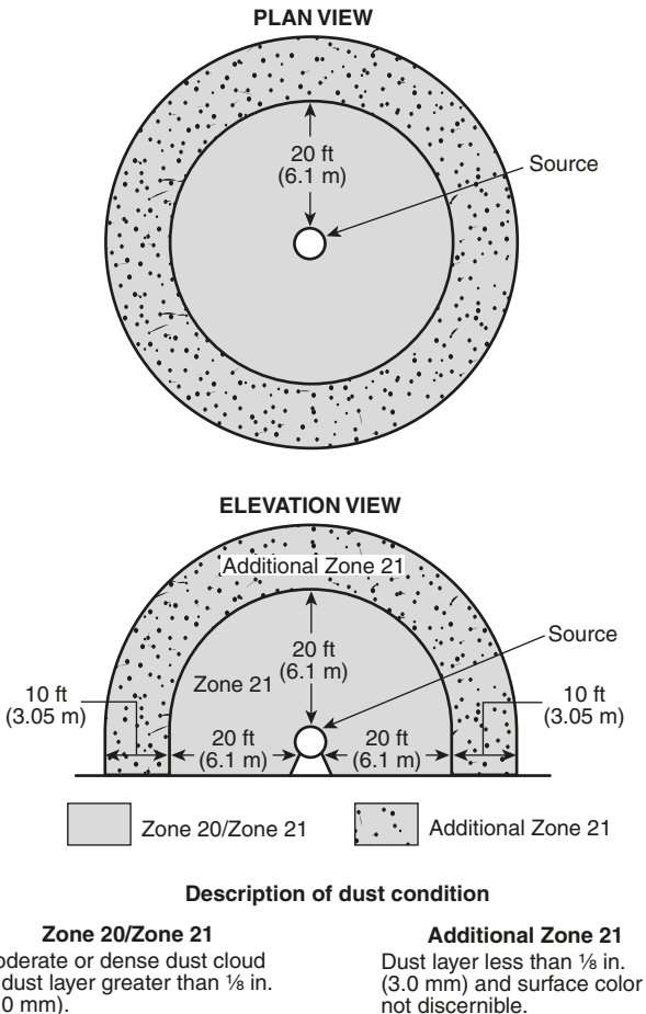
FIGURE 6.10(k) Zone Group IIIC Dust — Indoor, Unrestricted Area; Open or Semi-Enclosed Operating Equipment.
