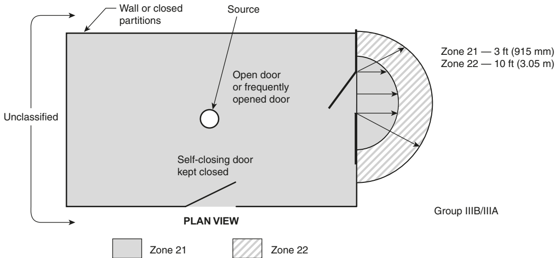
▲ FIGURE 6.10(o) Zone Group IIIC Dust — Indoor, Walled-Off Area; Operating Equipment Enclosed.
