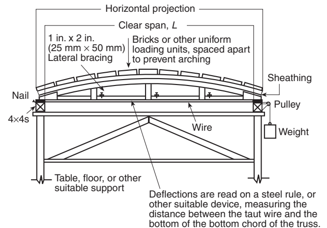
Figure 5-2.3 Nondestructive test procedure for roof trusses.
