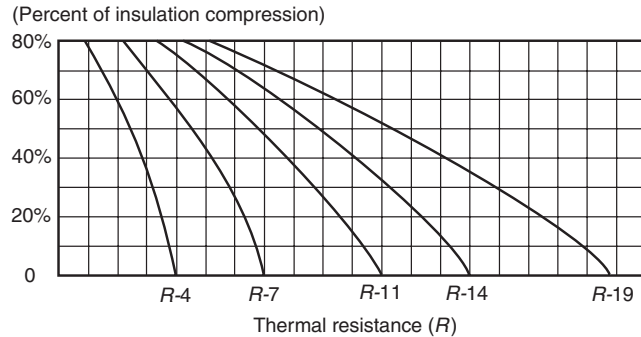
Figure 6-9.3 Thermal resistance graph showing reduction of insulation R -values when insulation is compressed.
