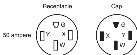
Figure 9-3.6 Receptacle and attachment plug cap configurations; 50-ampere 125/250-volt receptacle and attachment plug cap configurations, 3-pole, 4-wire, grounding types used for manufactured home supply cords and manufactured home parks. Complete details of the 50-ampere cap and receptacle can be found in the American National Standard Dimensions of Caps, Plugs and Receptacles, Grounding Type (ANSI C73.17-1972).
