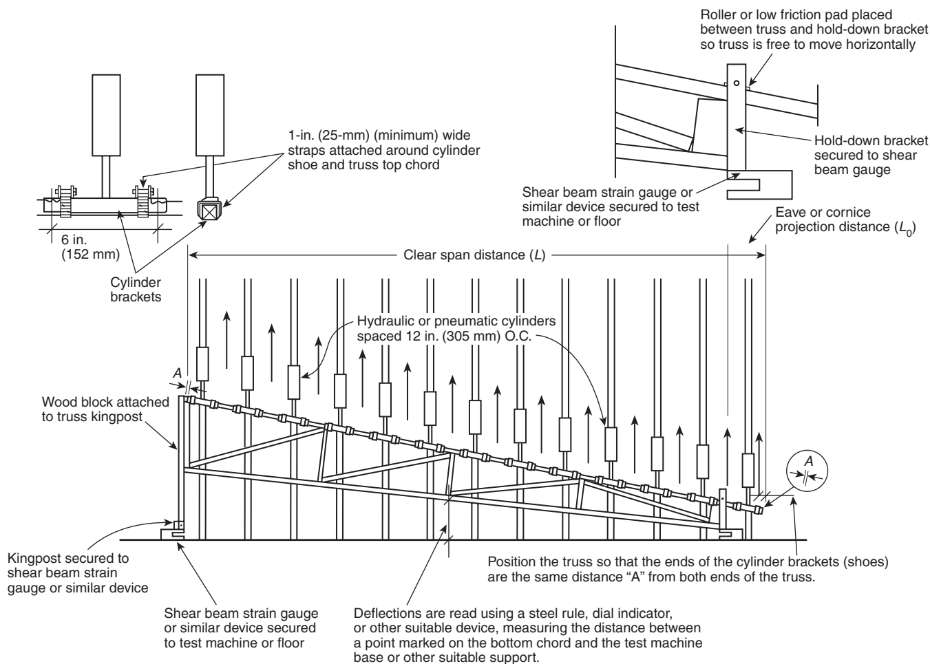
FIGURE 7.2.5.1 Uplift Load Test Fixture.
