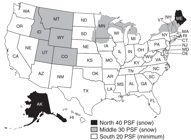
FIGURE 6.5.3.3.1 Roof Load Zone Map.
