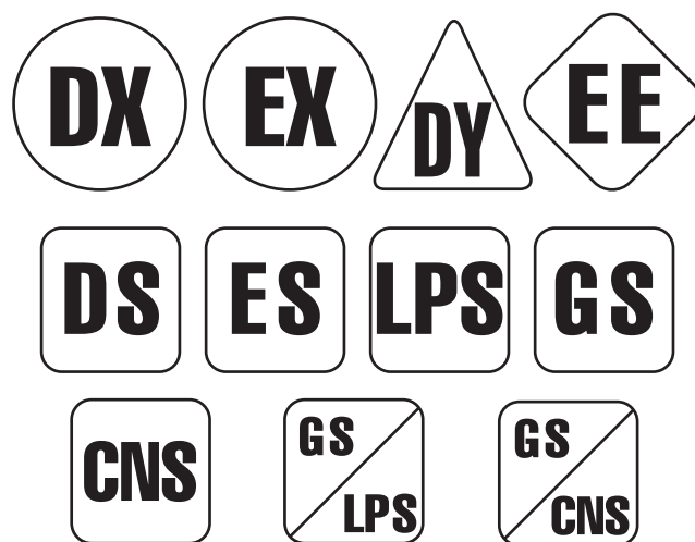
FIGURE 8.4.1.2.1 Markers Used to Identify Type of Industrial Truck.
