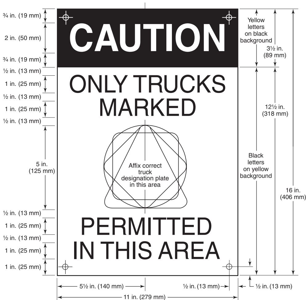
FIGURE 8.4.1.3 Building Sign for Posting at Entrance to Hazardous Areas.
