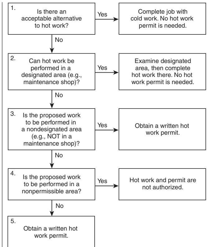
FIGURE A.5.3 Hot Work Permit Decision Tree.
