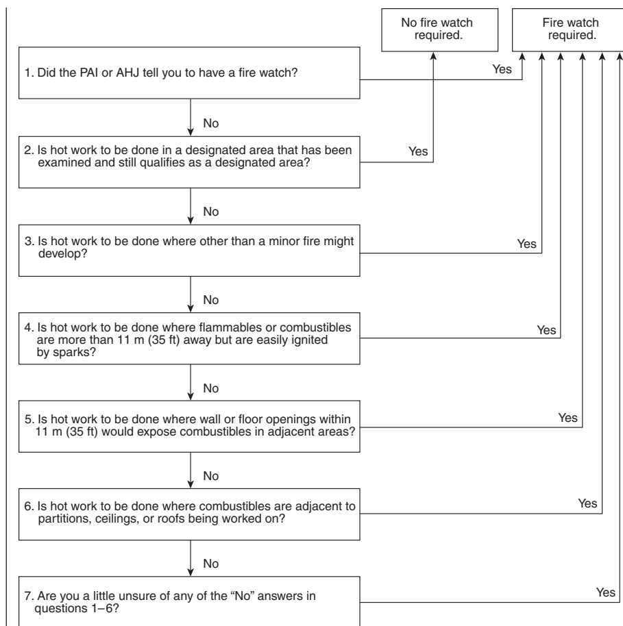
FIGURE A.5.4.1 Fire Watch Decision Tree.
