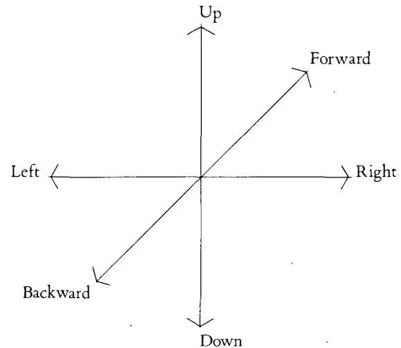
Figure 3-3.3 The Six Principal Directions.
