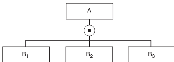
FIGURE 4.2.2(a) An Example of an “And” Gate.
