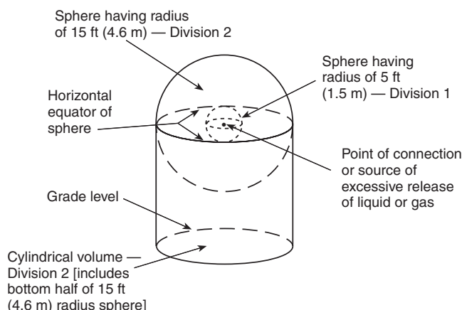
FIGURE A.4.5.2.2 Extent of Electrically Classified Area. (See Table 4.5.2.2.) [58:Figure A.6.22.2.3]
