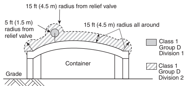
FIGURE 11.9.2(d) Full and Membrane Containment Tank Systems.
