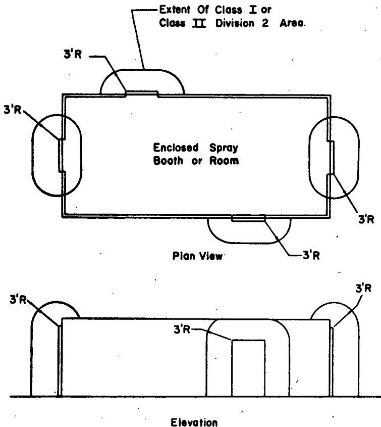
Figure 3.2 Class I or Class II, Division 2 Locations Adjacent to Openings in an Enclosed Spray Booth or Room
