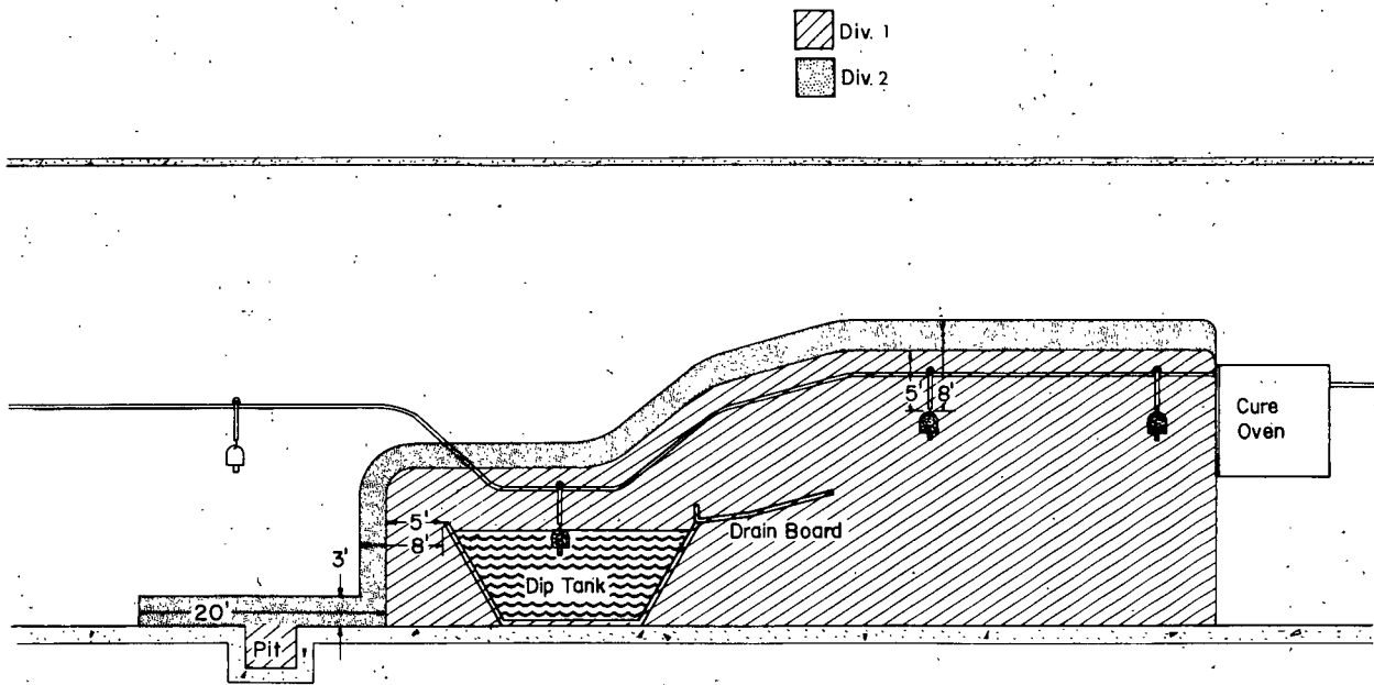
Figure 4.* The Extent of Class I, Division 1 and Class I, Division 2 Hazardous (Classified) Locations for a Paint Dipping Operation.
