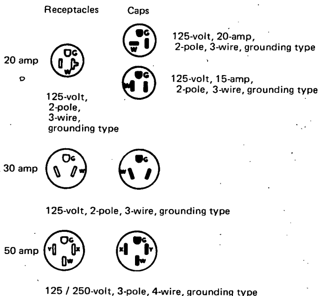
Figure 551-15(c). Configurations for grounding-type receptacles and attachment plug caps used for recreational vehicle supply cords and recreational vehicle lots.
