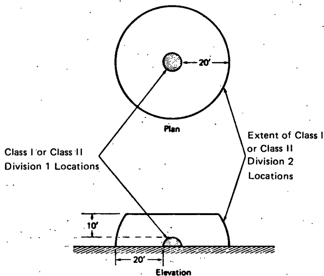
Figure 1.* Class I or Class II, Division 2 Locations Adjacent to an Unenclosed Spray Operation.
