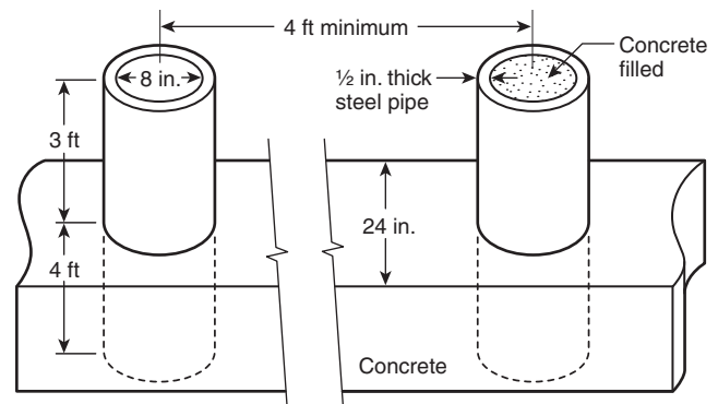
FIGURE E.2.1.2.1 Concrete-Filled Bollard. (Source: U.S. Army Corps of Engineers, Field Manual 19-30.)
