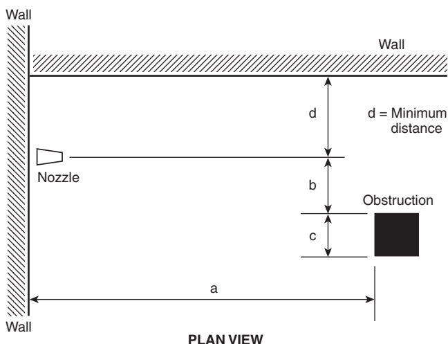
FIGURE A.8.2.5(g) Dimensional Considerations for Locating a Horizontally Discharging Water Mist Nozzle with Respect to an Obstruction in the Spray Path, Such as a Column or a Parallel Wall.
