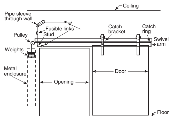
FIGURE A.4.7.5(e) Closing Devices for Single Sliding Door (Level Track).
