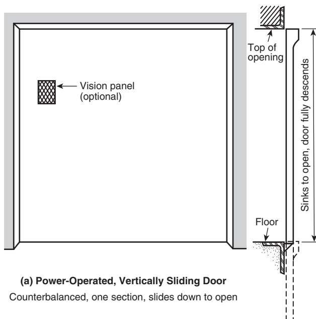
FIGURE A.14.2.3(a) Power-Operated, Vertically Sliding Door and Hand- or Power-Operated, Vertically Sliding Door. (Courtesy of ASME A17.1 Handbook on Safety Code for Elevators and Escalators.)
