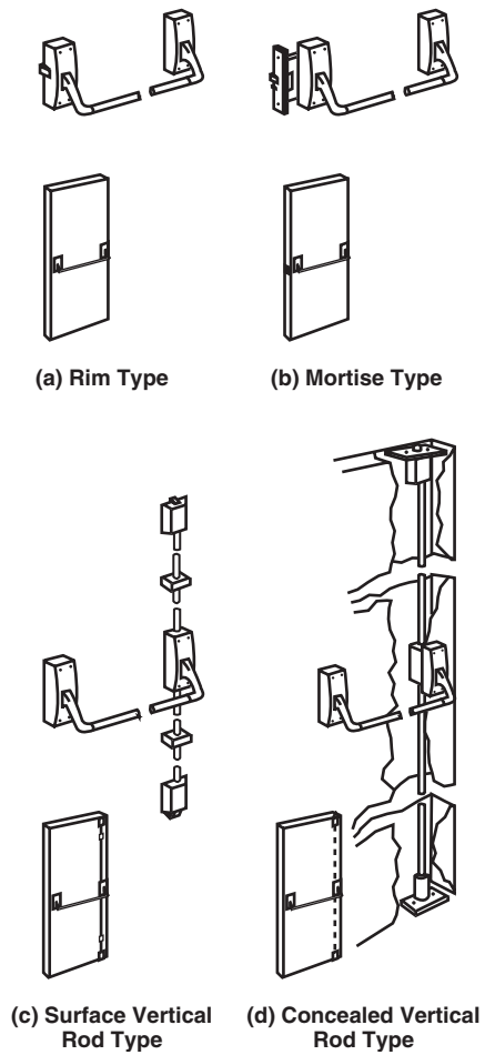
FIGURE A.4.6.3.1(e) Types of Fire Exit Hardware.
