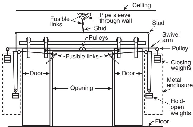
FIGURE A.4.7.5(g) Closing Devices for Center-Parting, Horizontally Sliding Doors (Level Track).
