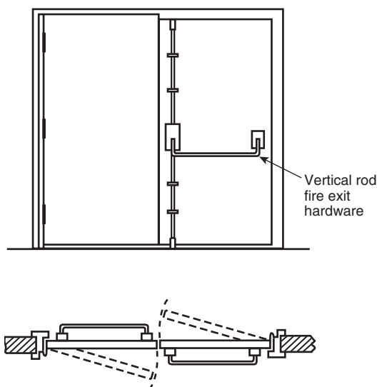
FIGURE A.3.3.45 Double Egress Door and Frame.
