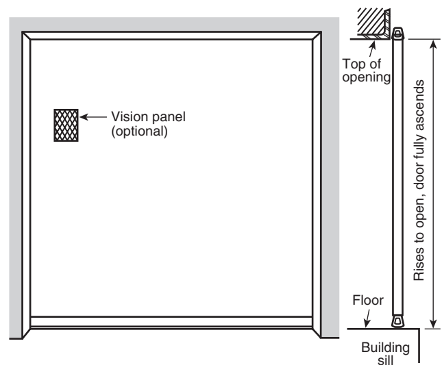
(b) Hand- or Power-Operated, Vertically Sliding Door Counterweighted, one section, slides up to open
