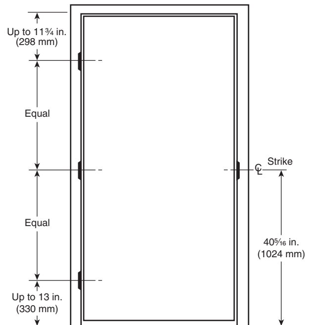
FIGURE F.2(a) Swinging Wood Composite Fire Doors Equipped with Builders Hardware.
