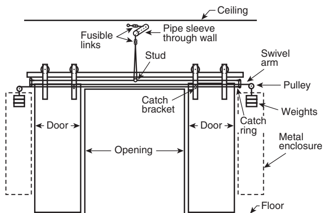
FIGURE A.4.7.5(h) Closing Devices for Center-Parting, Horizontally Sliding Doors (Level Track).
