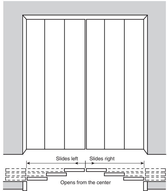
(b) Center-Parting, Horizontal Slide Doors Multiple sections, multiple speeds
