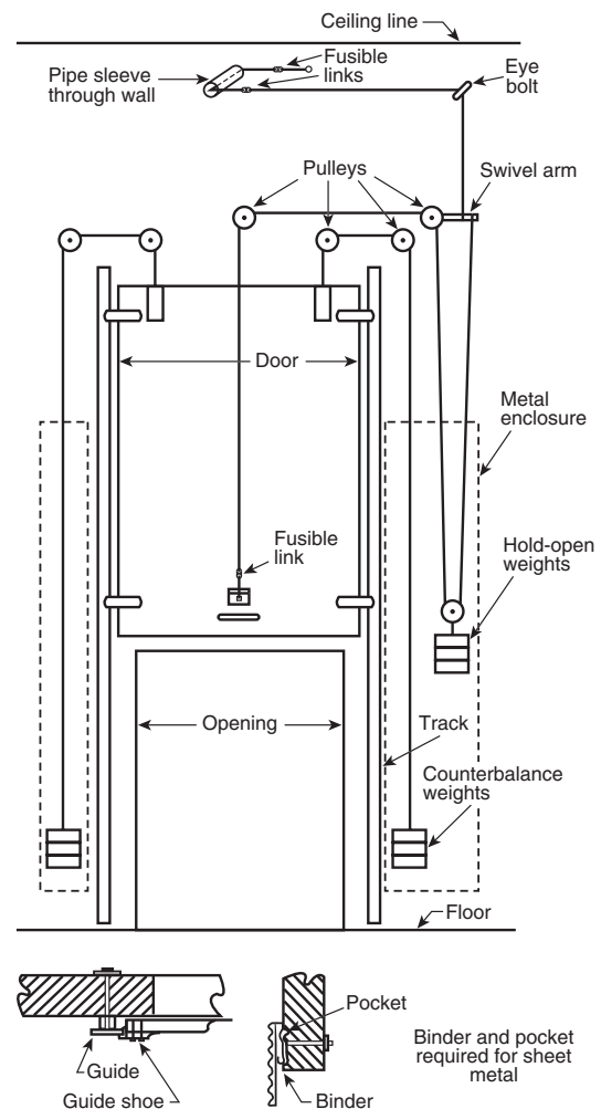
FIGURE A.4.6.4(h) Vertically Sliding Door.
