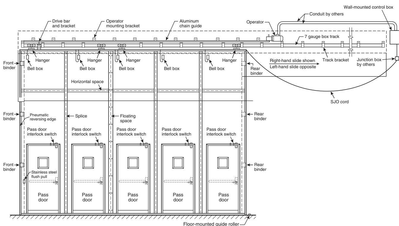
FIGURE A.8.1.2.7(c) Combination Swinging Pass Door and Sliding Door — Arrangement C.
