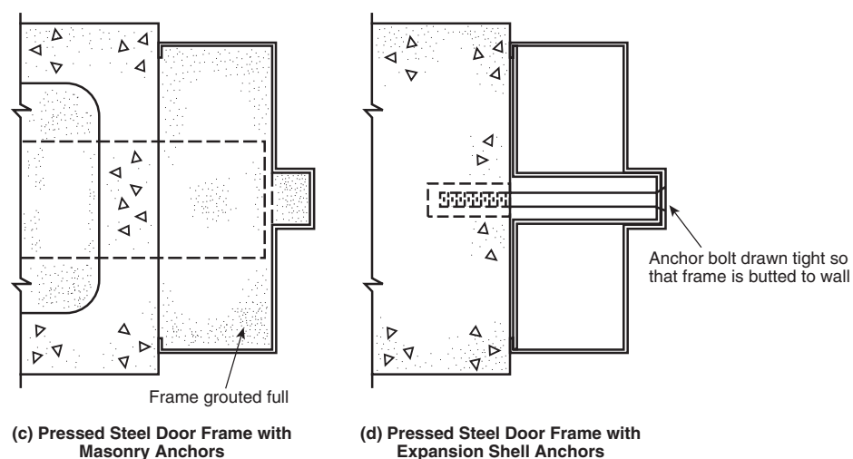
FIGURE A.4.6.3.1(g) Typical Pressed Steel Door Frame Installations.
