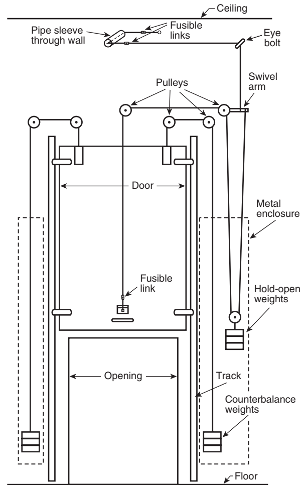
FIGURE A.4.7.5(i) Closing Devices for Vertically Sliding Door.
