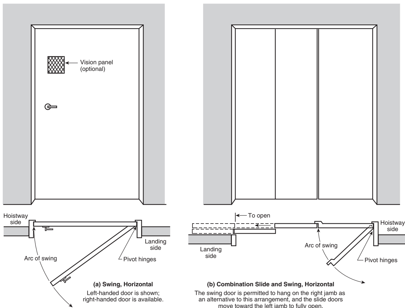
FIGURE A.14.2.1.3 Horizontal Swinging and Horizontal Combination Sliding and Swinging Doors. (Courtesy of ASME A17.1 Handbook on Safety Code for Elevators and Escalators.)
