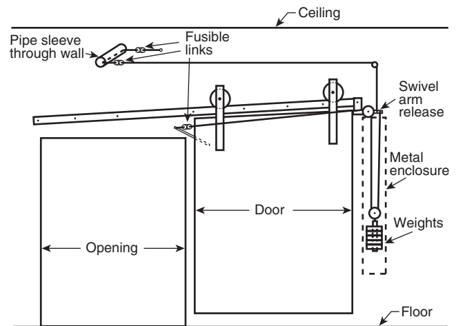
FIGURE A.4.7.5(c) Closing Devices for Single Sliding Door (Inclined Track).
