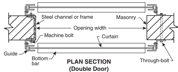
FIGURE A.4.7.5(k) Rolling Steel Doors — Surface Mounted.
