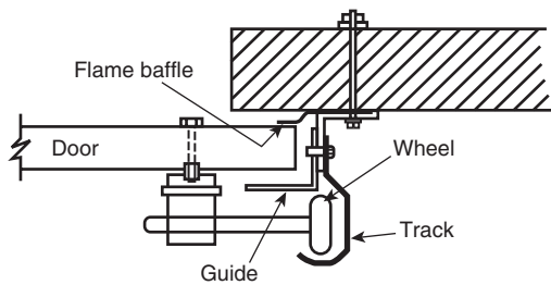
FIGURE A.4.7.5(j) Vertically Sliding, Steel-Sectional Overhead Door.
