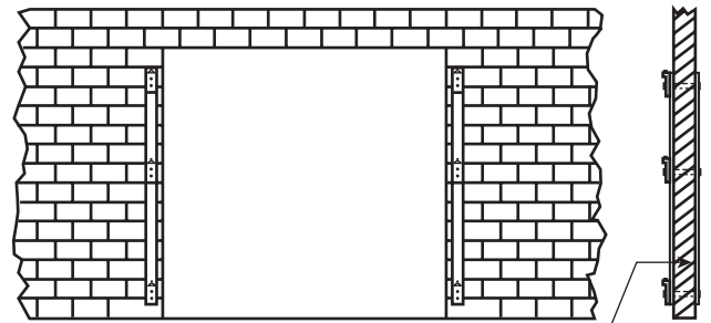
FIGURE A.4.8.1.4 Hollow Concrete Masonry Wall Prepared for Doors Swinging in Pairs — Lap Mounted.
