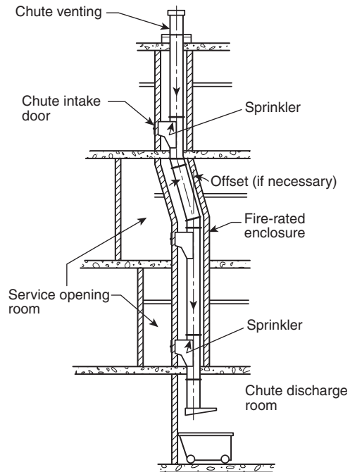
Gravity Chute with Offset Only When Necessary by Building Conditions and with Approval of AHJ
