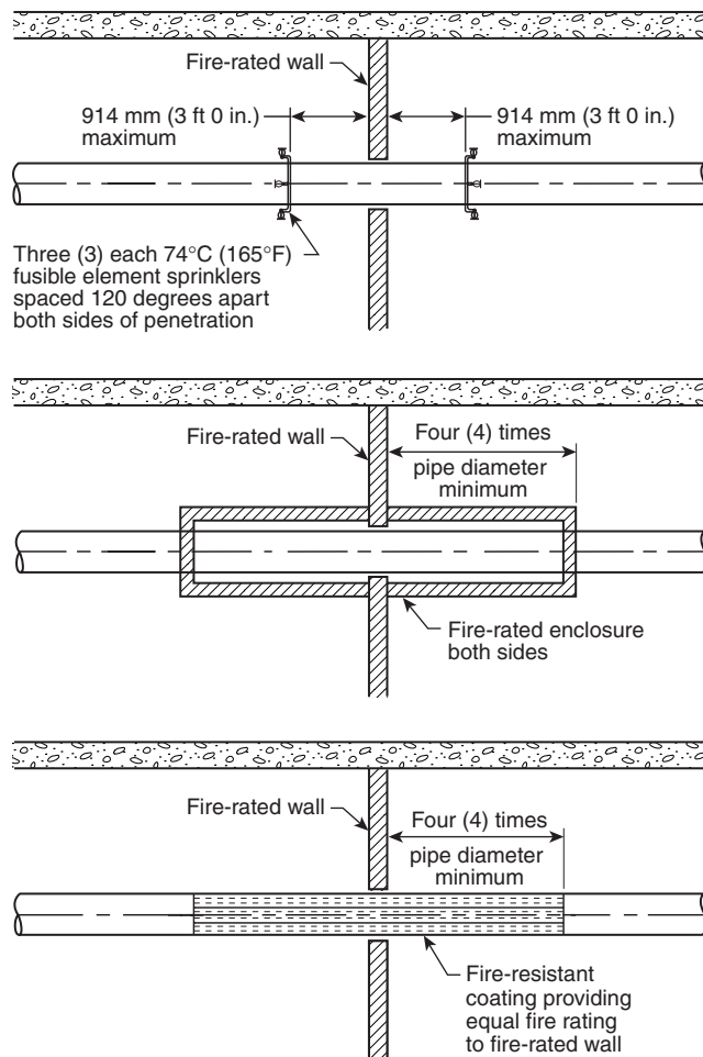
FIGURE A.5.3(d) Fire Damper Engineering Alternative for Penetration of Fire-Rated Wall.
