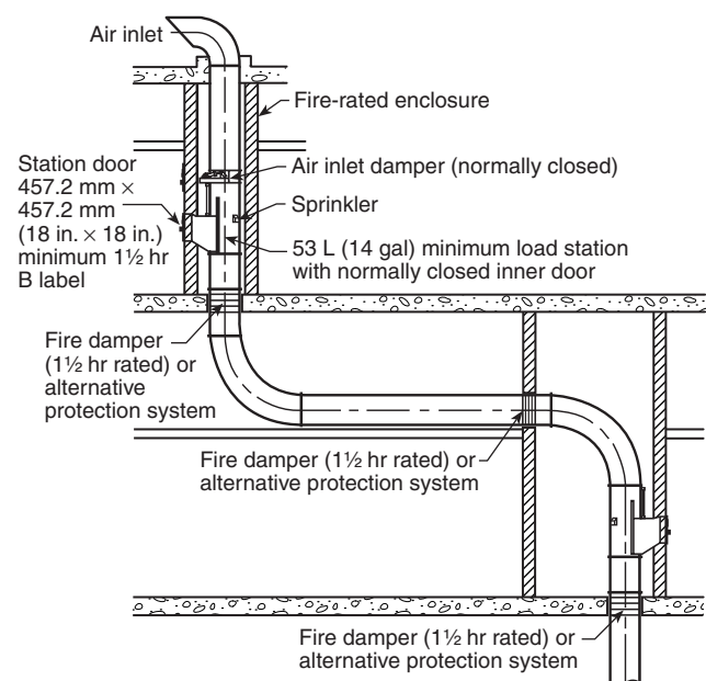
FIGURE 5.3.5.2.1(a) Full Pneumatic Riser with Offset.
