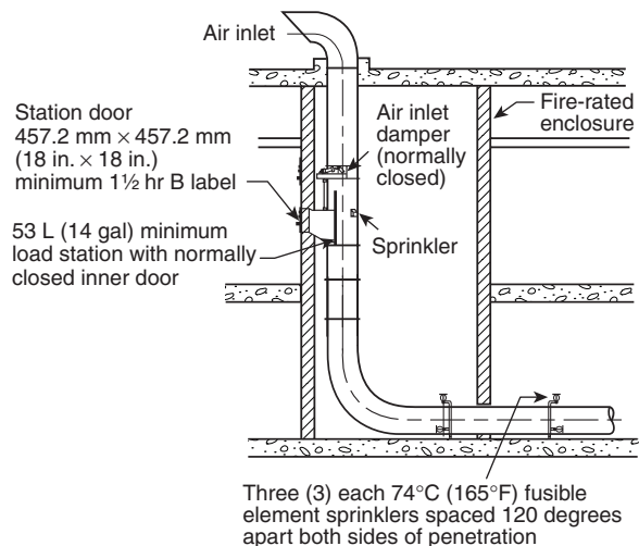
FIGURE A.5.3(e) Fire Damper Engineering Alternative for Penetration of Wall at Base of Shaft.
