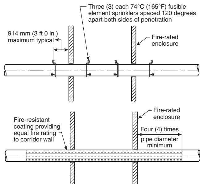
FIGURE A.5.3(c) Fire Damper Engineering Alternative for Penetration of Fire-Rated Enclosure.
