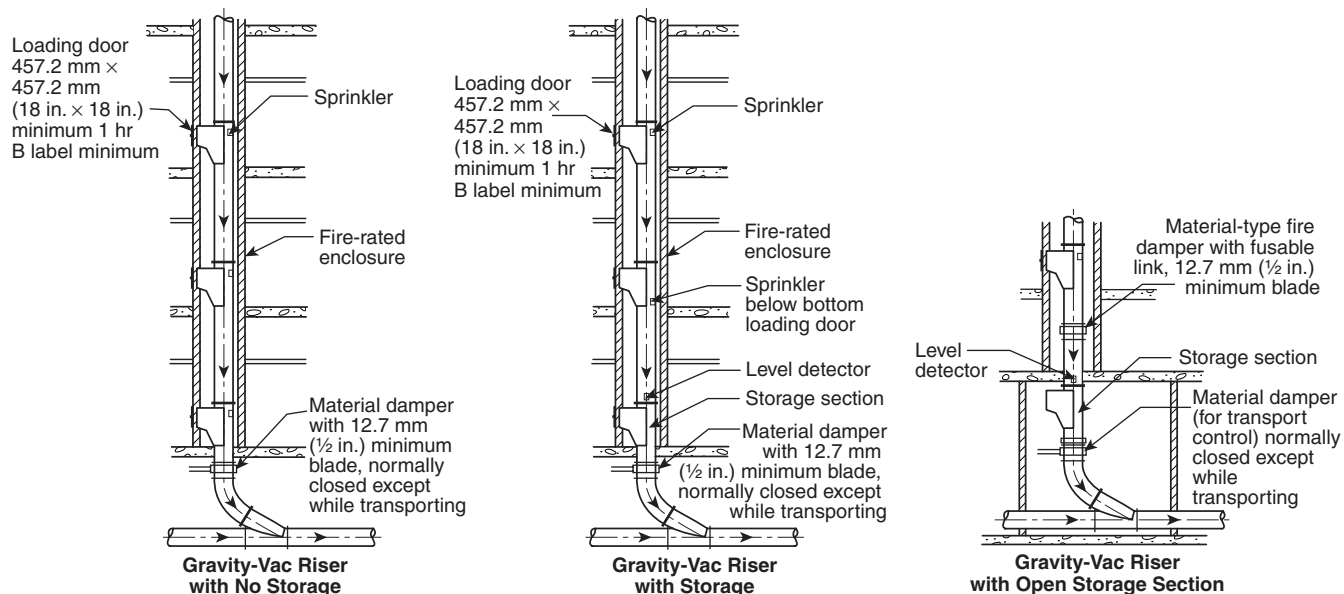
FIGURE A.5.4 Gravity Pneumatic System.
