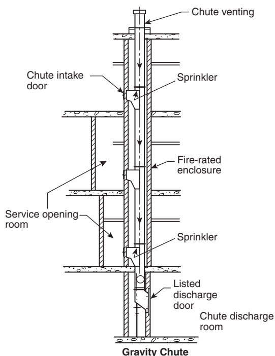
FIGURE A.5.2(a) Gravity Linen Chute.
