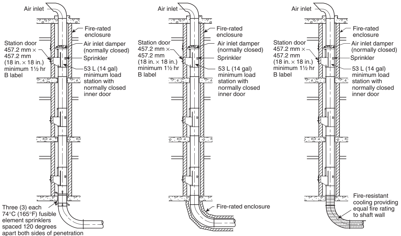
FIGURE A.5.3(b) Fire Damper Engineering Alternative for Penetration of Floor at Base of Shaft.
