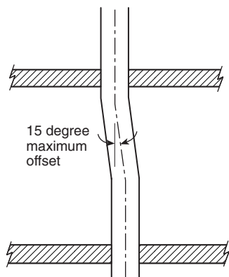
FIGURE 5.2.2.2 Gravity Metal Chute, Maximum Offset.
