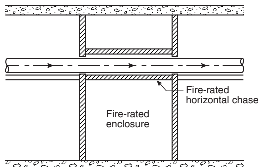
FIGURE 5.3.5.2.1(b) Full Pneumatic System with Penetration of an Evacuation Corridor.
