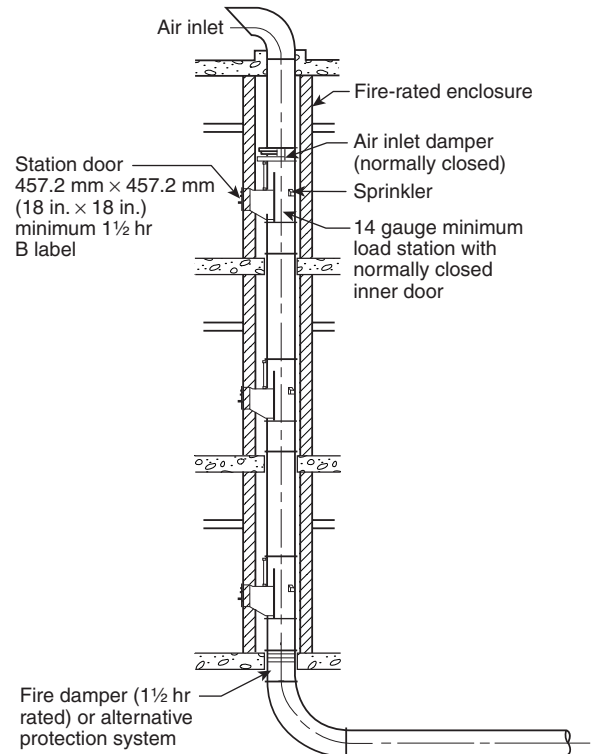
FIGURE A.5.3(a) Full Pneumatic System.
