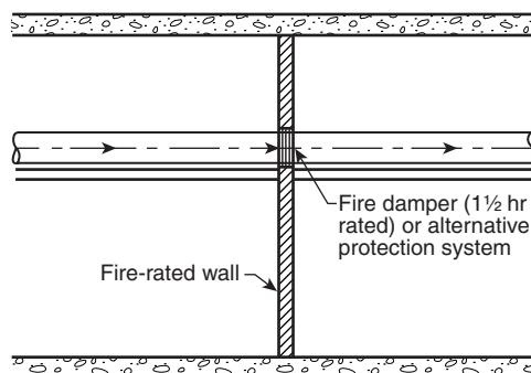
FIGURE 5.3.5.2.1(c) Full Pneumatic System with Penetration of a 2-Hour Fire-Rated Wall.
