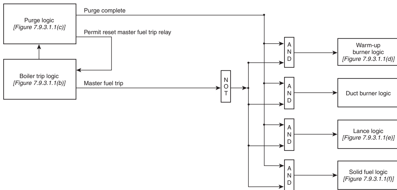
FIGURE 7.9.3.1.1(a) Interlock Overview.
