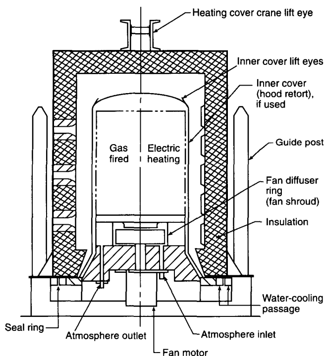
Figure 12-1.2.1 Example of a bell-type furnace.
