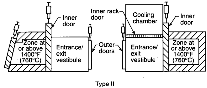
Figure 9-2.4.1 Example of Type II special processing atmosphere furnace.
