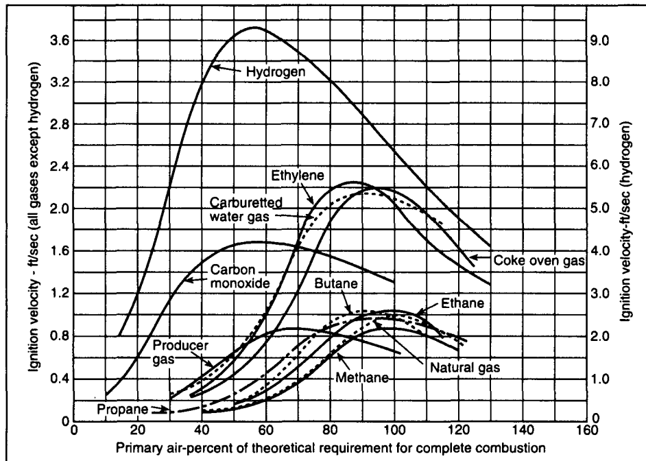
Figure A-4-2.1.1 Ignition velocity curves for typical flammable gases.
