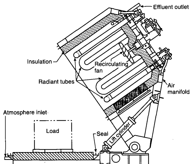
Figure 12-1.2.2 Example of a tip-up-type furnace.
