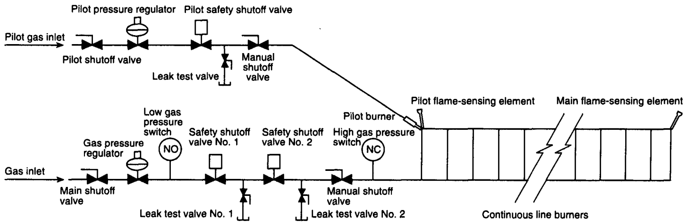
Figure A-5-9.2.2(a) Example of an approved combustion safeguard supervising a pilot for a continuous line burner during light-off and the main flame alone during firing.
