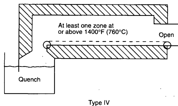
Figure 10-2.4.1 Example of Type IV special processing atmosphere furnace.
