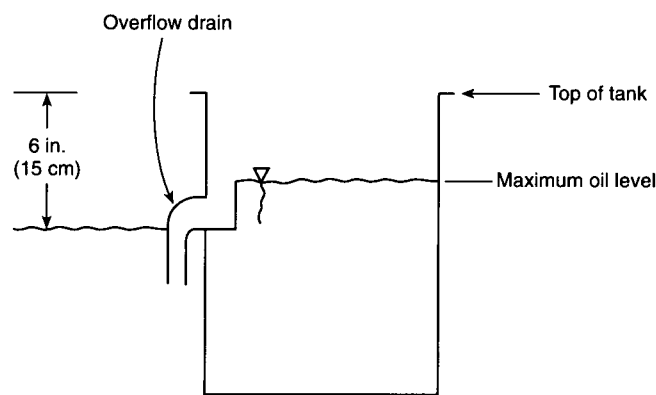
Figure 14-7.3.1 Example of overflow drains for open integral quench tanks.
