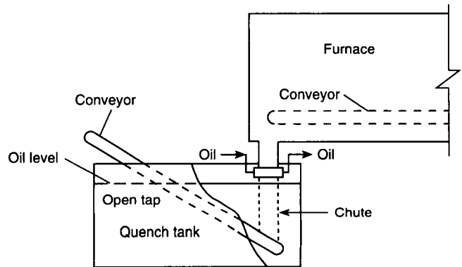
Figure 14-2 Example of integral quench furnace Type QIII.
