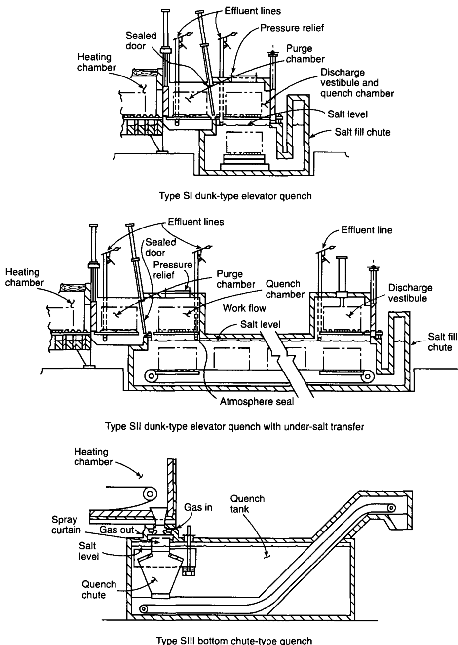
Figure 16-7.1 Examples of integral quench tanks.
