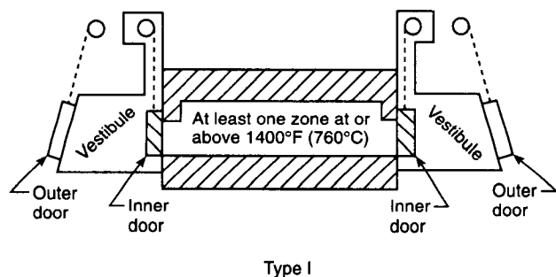
Figure 9-2.2.1 Example of Type I special processing atmosphere furnace.
