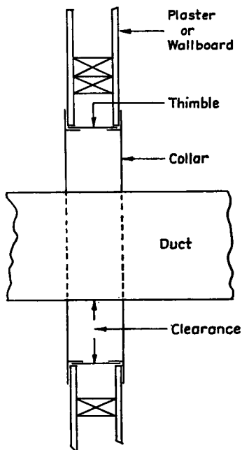
Figure 4. An arrangement for passing ducts through combustible walls or partitions as specified in par. 143 c.
