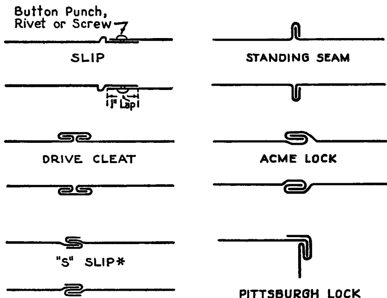
Fig. 1. Types of duct joints.
