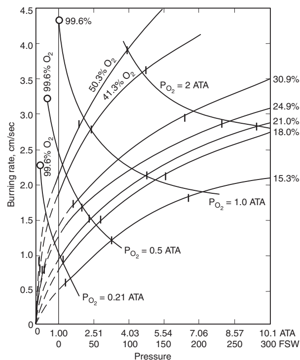
Δ FIGURE A.3.3.3.3 Burning Rates of Filter Paper Strips at an Angle of 45 Degrees in N 2 -O 2 Mixtures. (Adapted from Figure 4 of “Technical Memorandum UCRI-721, Chamber Fire Safety.”)
