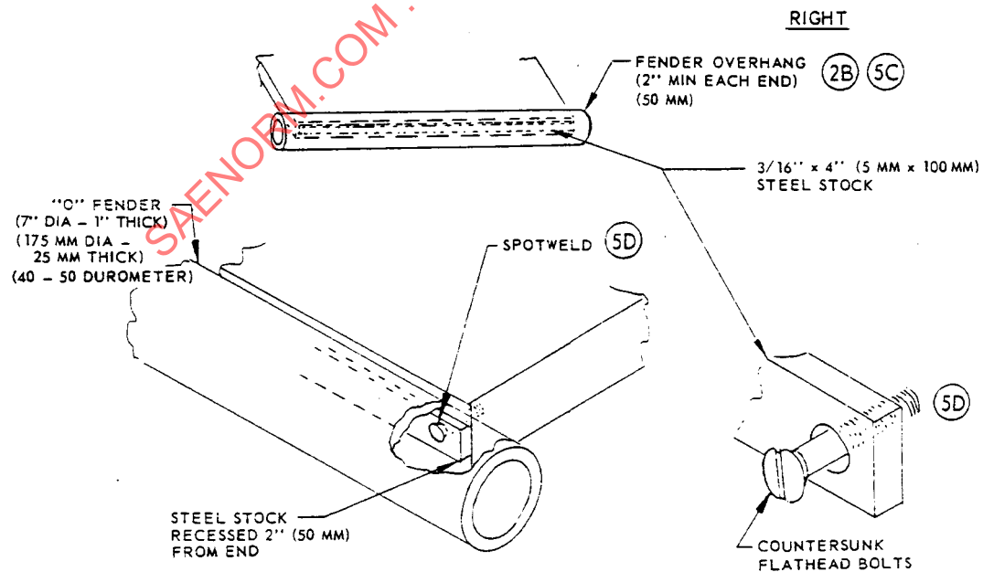
FIGURE 1 - Basic Fender Installation
