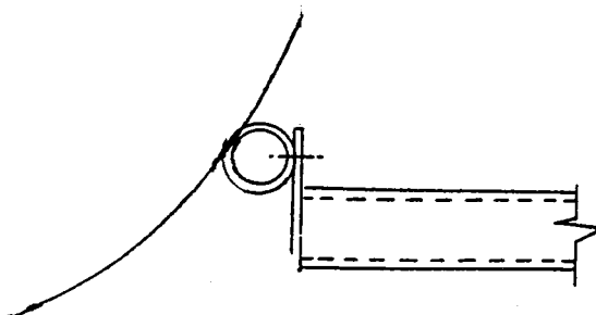
FIGURE 2 - Example of Correct Placement of Bumpers or Fenders
