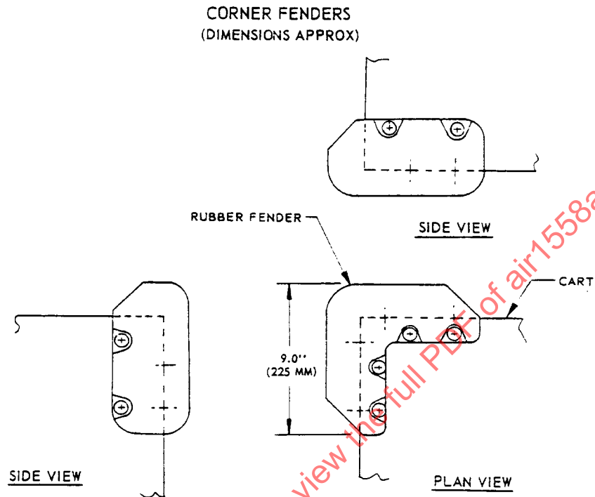
FIGURE 5 - Corner Fenders (Dimensions Approximate)
