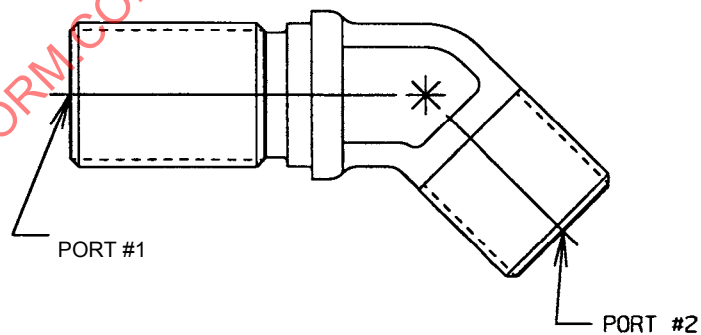
FIGURE 4 - FITTING, ELBOW, 45°, BULKHEAD END NOT FOR USE IN PORT INSTALLATION, NON-REDUCER SHOWN, SAME AS FIGURE 2 EXCEPT AS SHOWN
