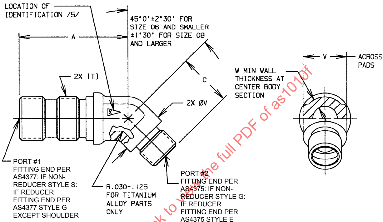
FIGURE 1 - FITTING, ELBOW, 45°, BULKHEAD END FOR OPTIONAL USE IN PORT INSTALLATION. PORT #1 SHOWN AS NON-REDUCER, PORT #2 SHOWN AS REDUCER
