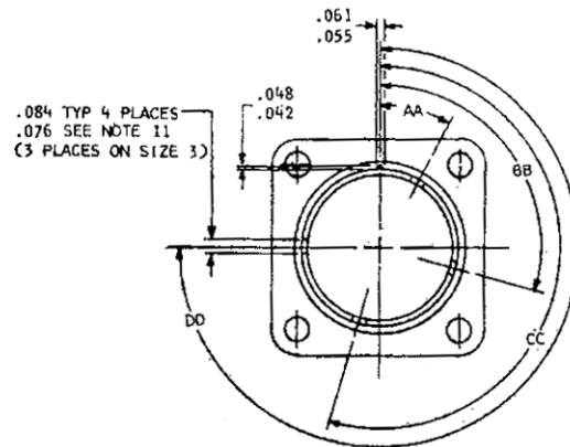
FIGURE 11 KEYWAY POSITIONS
