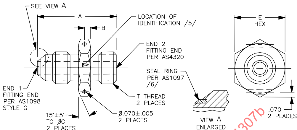
FIGURE 1 - FITTING, FLARED TO EXTERNAL STRAIGHT THREAD
