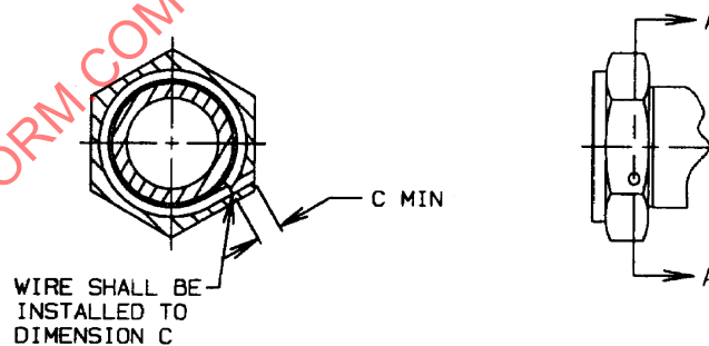
FIGURE 1 - ELBOW ASSEMBLY, 90°
