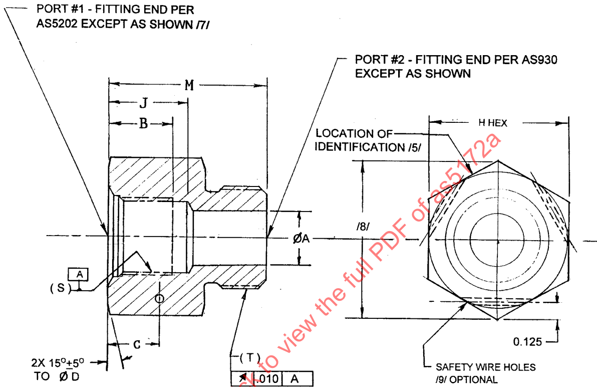
FIGURE 1 - FITTING-ADAPTER
