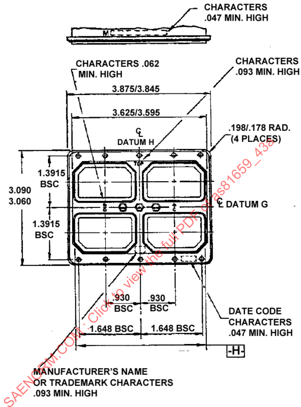
FIGURE 2 – CONNECTOR CONFIGURATIONS AND DIMENSIONS
