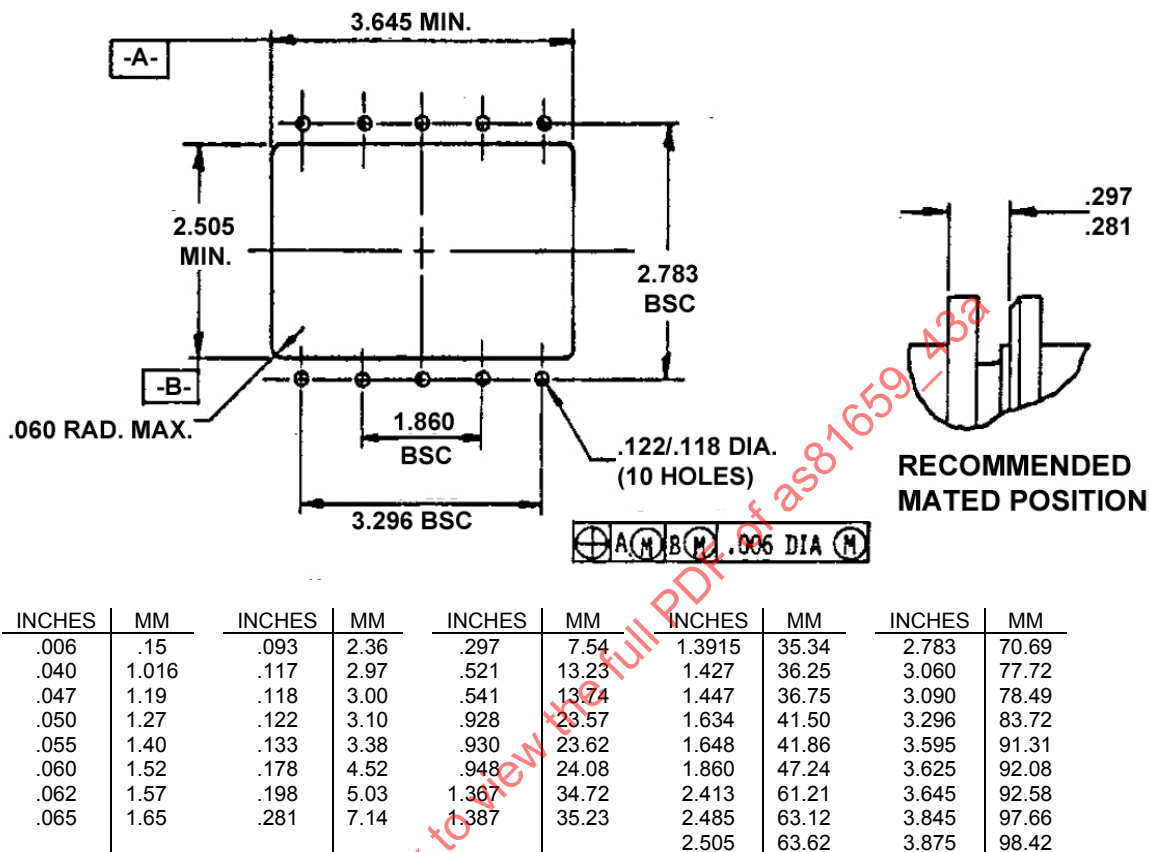
FIGURE 1—SUGGESTED PANEL CUT-OUT DIMENSIONS
