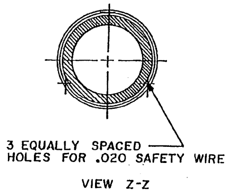
FIGURE 2 – SAFETY WIRE HOLES
