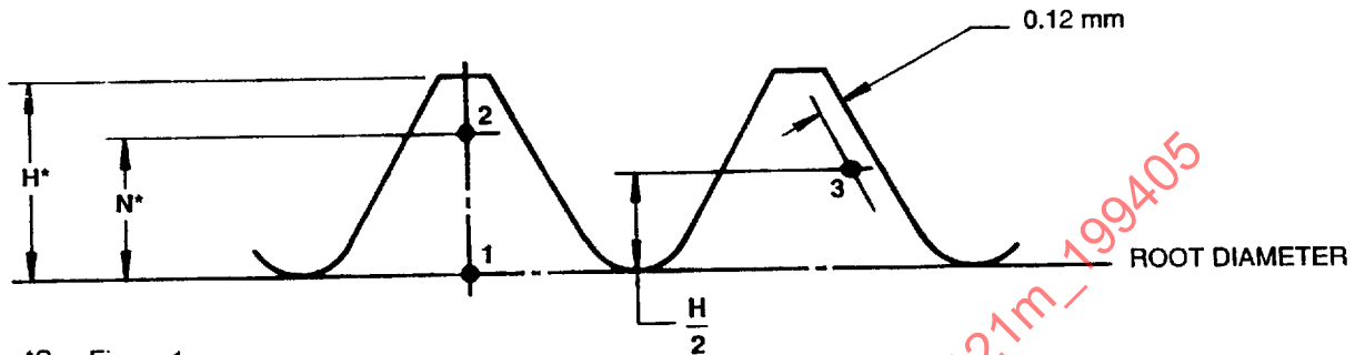
FIGURE 2—POSITIONS FOR DETERMINING HARDNESS
