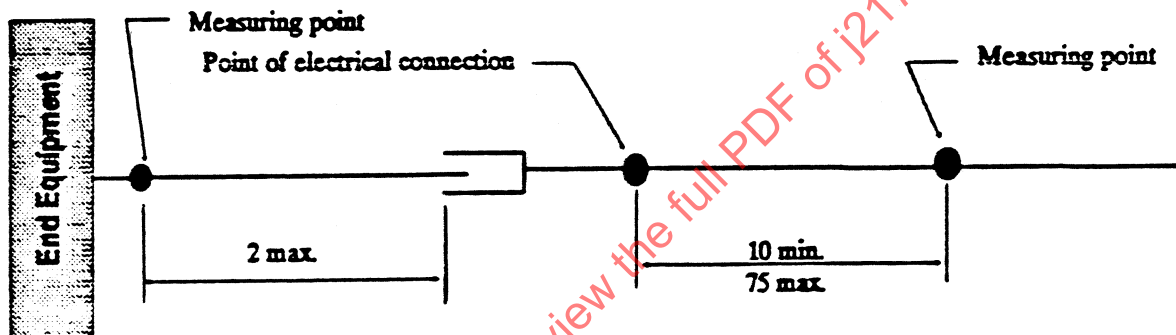
Figure 1 - Cable to cable assembly
