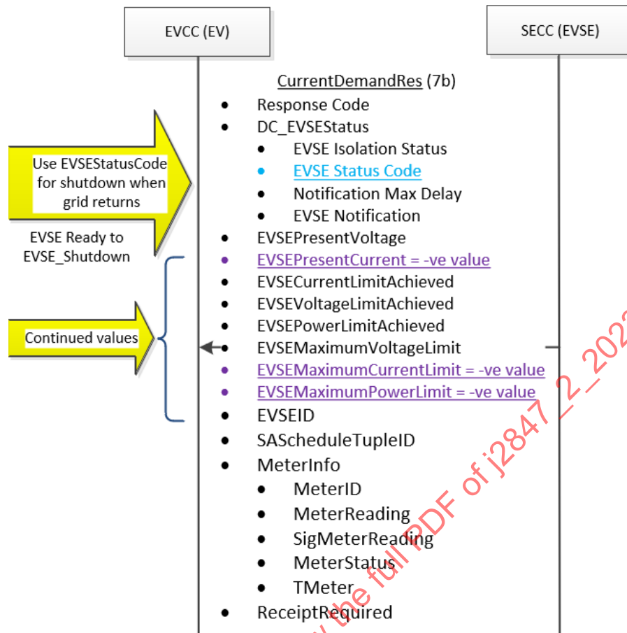
Figure 36 - CurrentDemand message
