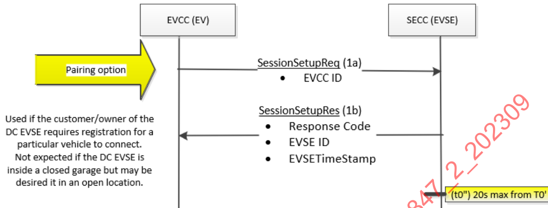
Figure 28 - Pairing signals
