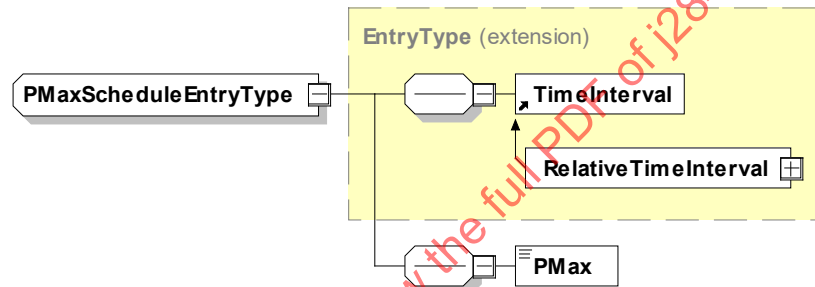
Figure 10 - Schema diagram—PMaxScheduleEntryType
