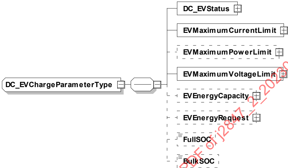
Figure 4 - Schema diagram—DC_EVChargeParameterType
