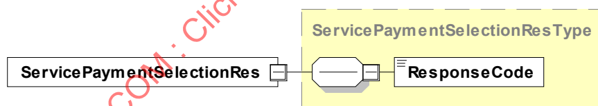
Figure 56 - Schema diagram—ServicePaymentSelectionRes
