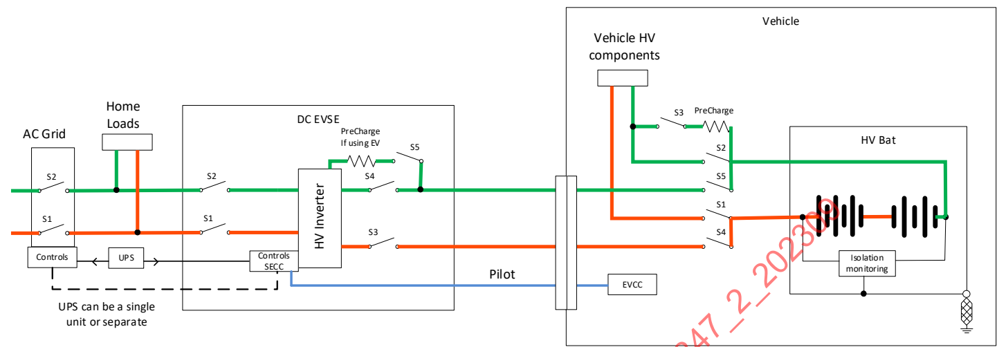
Figure 34 - Option 2 DC V2H system schematic
