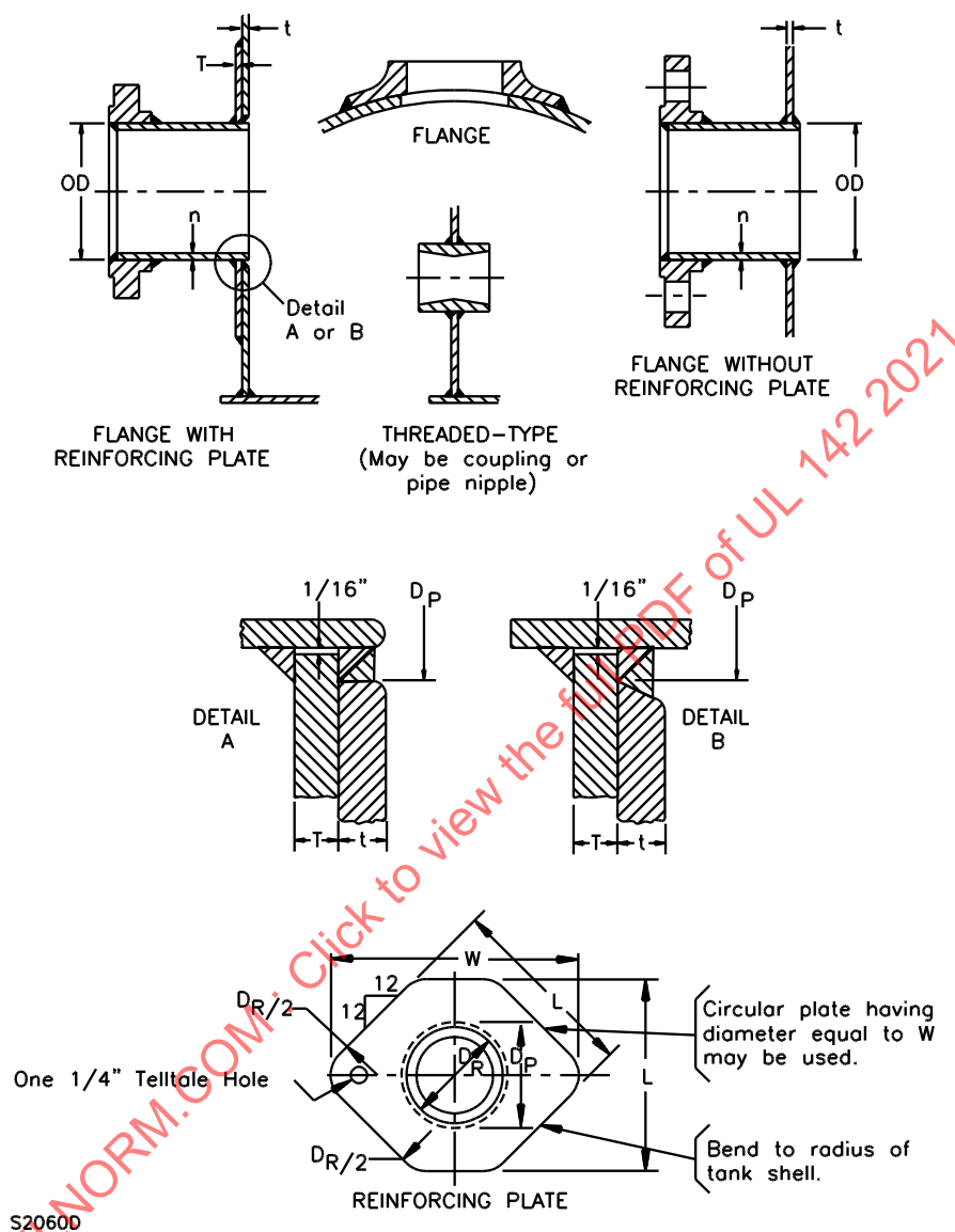
Figure 7.2 Top or shell connections (See Table 7.1)
