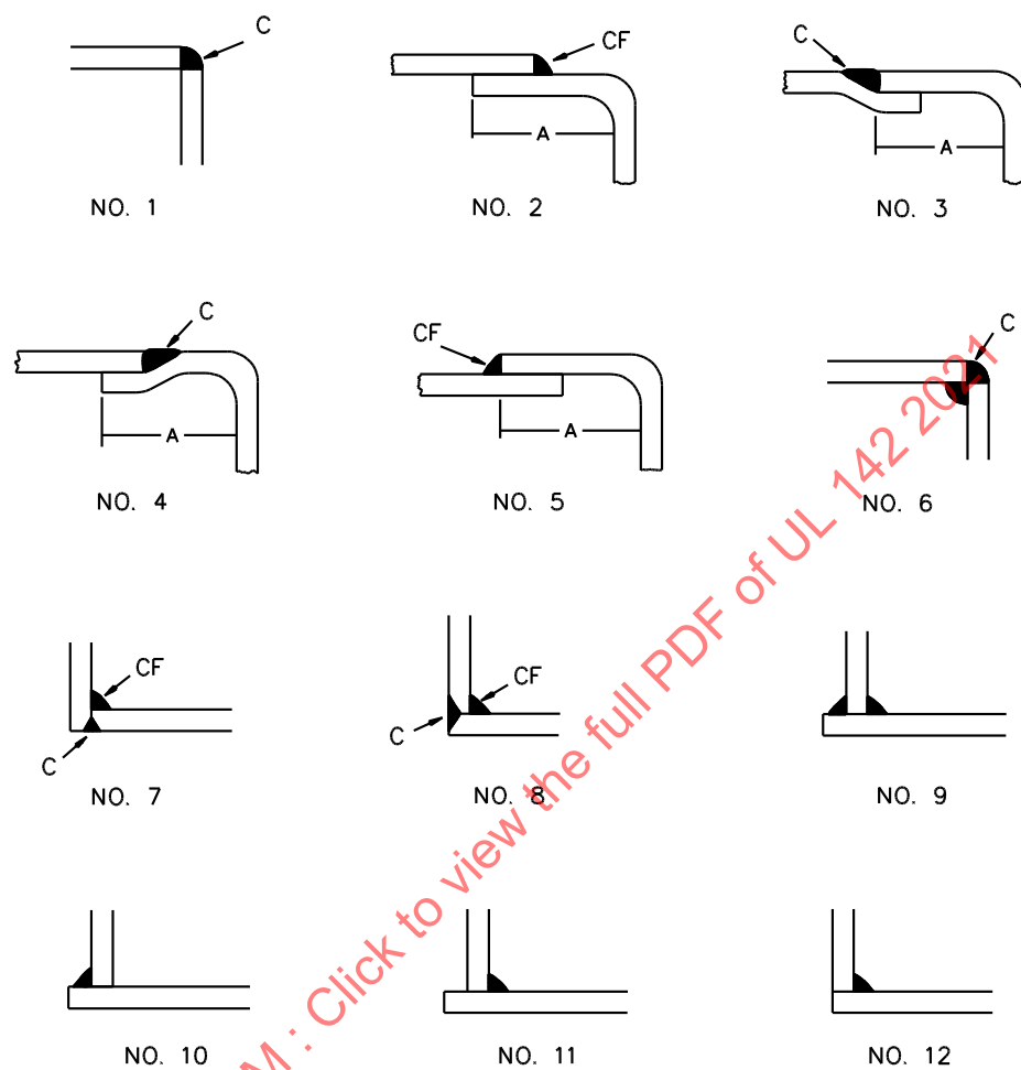
Figure 6.5 Corner joints
