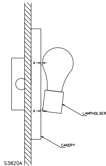
Figure 7.2.3.1 Minimum lamp spacings for wall-mounted luminaries
