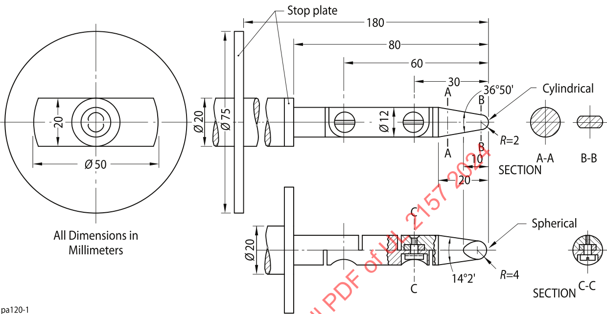
Figure 6.3 IEC Accessibility Probe with Stop Plate
