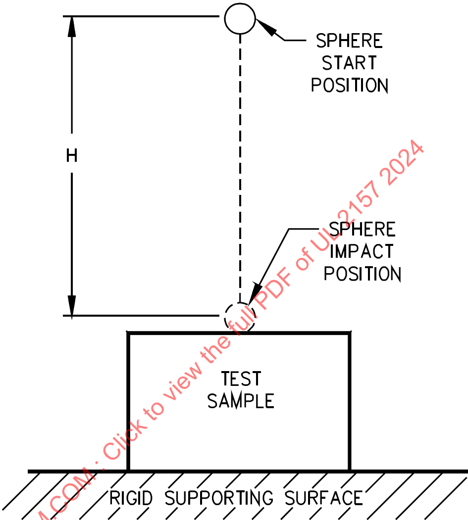
Figure 16.1 Ball Impact Test
