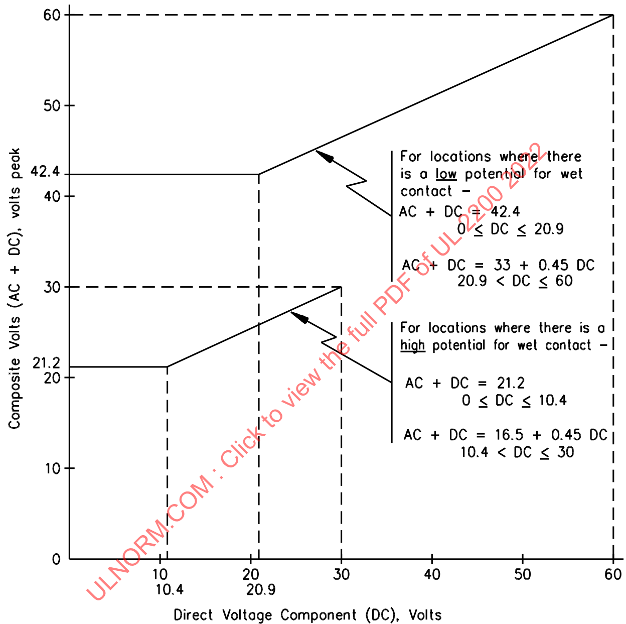
Figure 9.1 Maximum voltage
