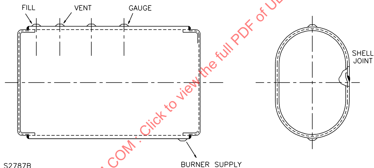
Figure 12.2 Typical obround storage tank
