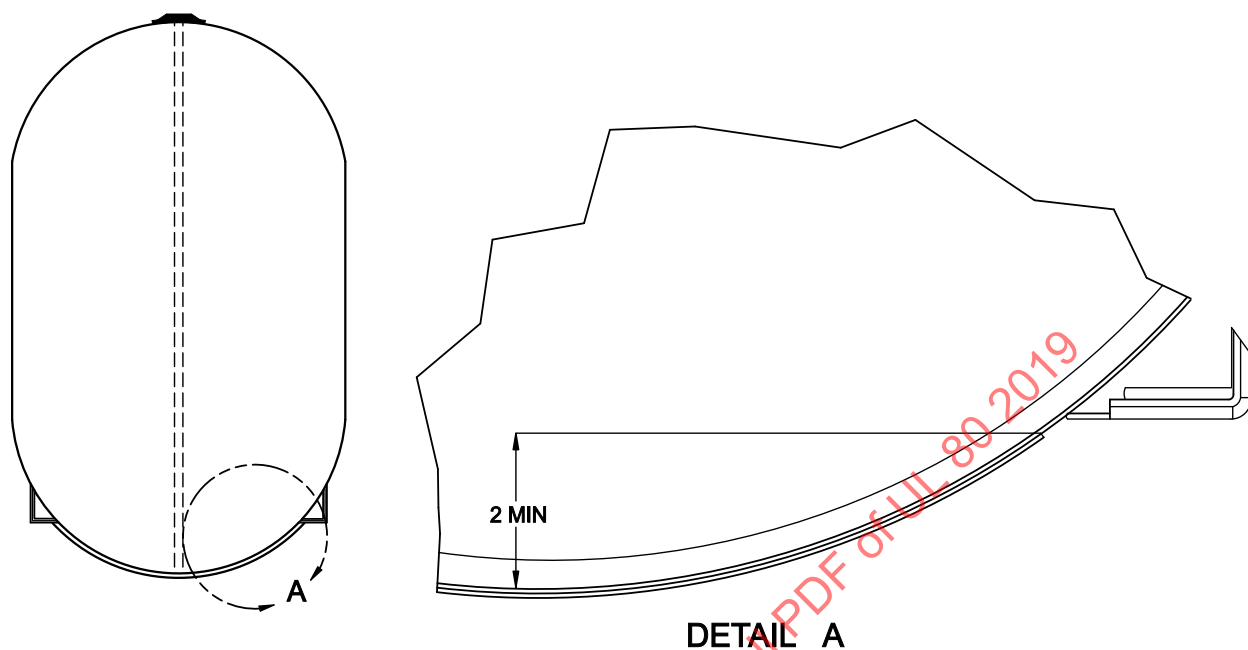
Figure 8.1 Typical double bottom obround tank – end view
