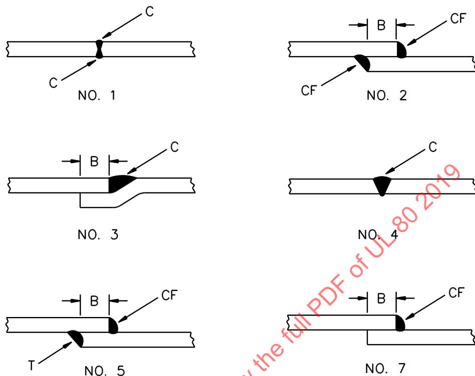
Figure 10.1 Shell seams
