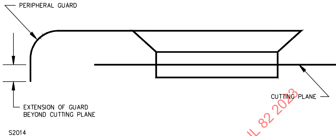
Figure 57.1 Extension of peripheral guard
