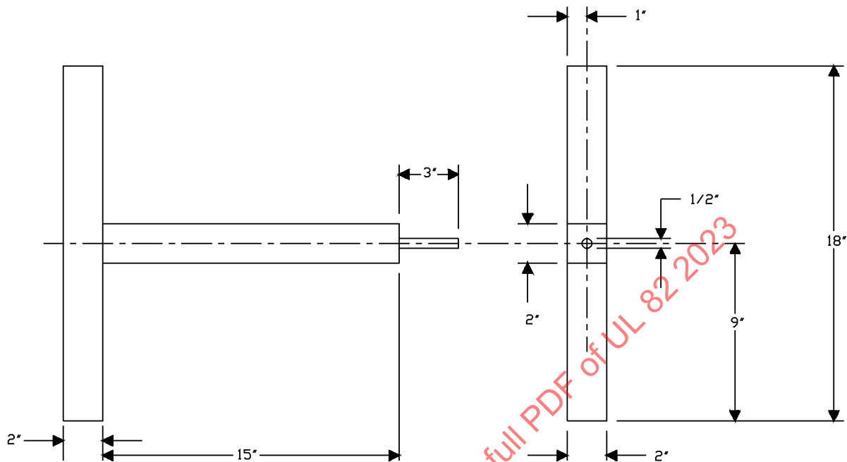
Figure 61.1 Arm probe
