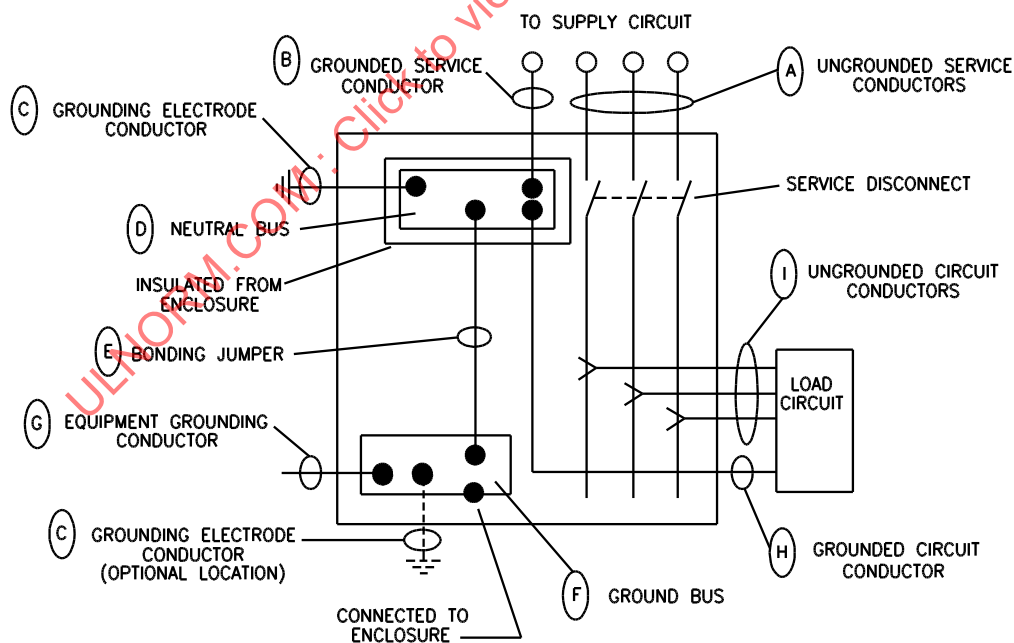
THREE PHASE, FOUR WIRE MOTOR CONTROL CENTER (THREE PHASE, FOUR WIRE DISTRIBUTION)
