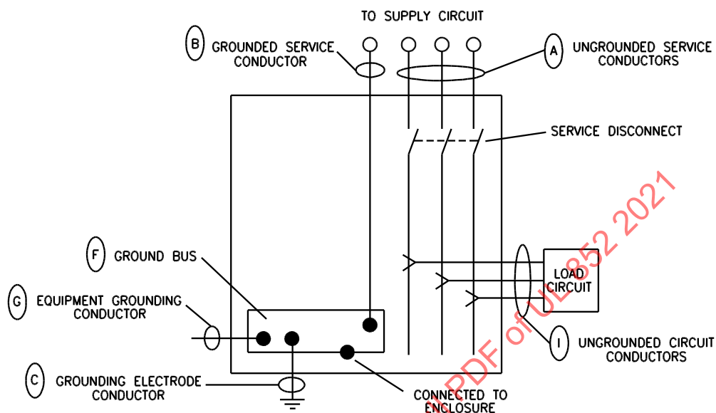
TYPICAL THREE PHASE, FOUR WIRE MOTOR CONTROL CENTER (THREE PHASE, THREE WIRE DISTRIBUTION)
