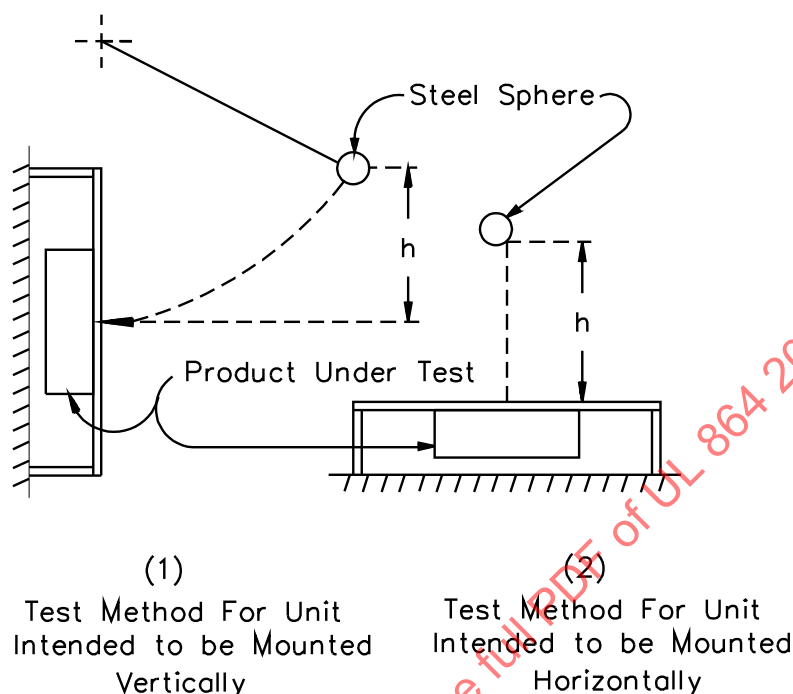
Figure 83.1 Jarring Test
